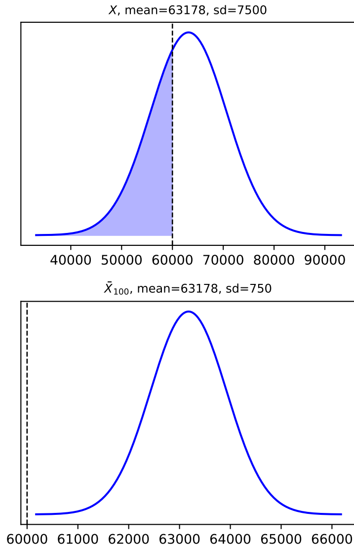
Figure 1: Salary distribution X (wide) vs. sample-average distribution \bar{X}_{100} (narrow), both with mean $63,178. The shaded left tail up to $60,000 is much larger for X ( \approx 0.34 ) than for \bar{X}_{100} ( \approx 0.0000133 ).
