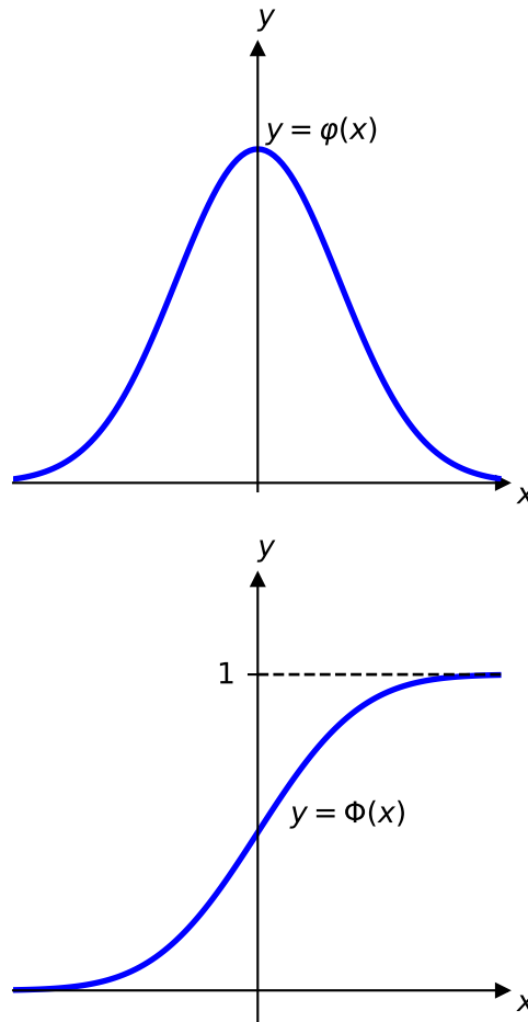
Figure 5: Functions \varphi(x) and \Phi(x)
