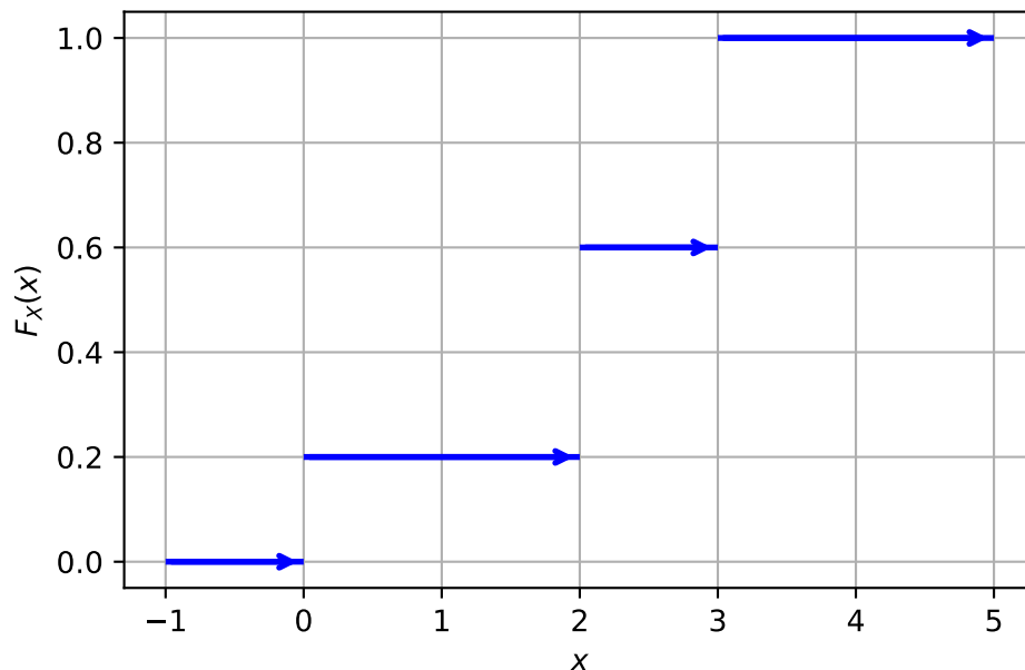
Figure 3.1: Cumulative function of the random variable X : \Omega \rightarrow \{0, 2, 3\} with \mathbb{P}(X = 0) = 0.2 , \mathbb{P}(X = 2) = \mathbb{P}(X = 3) = 0.4
