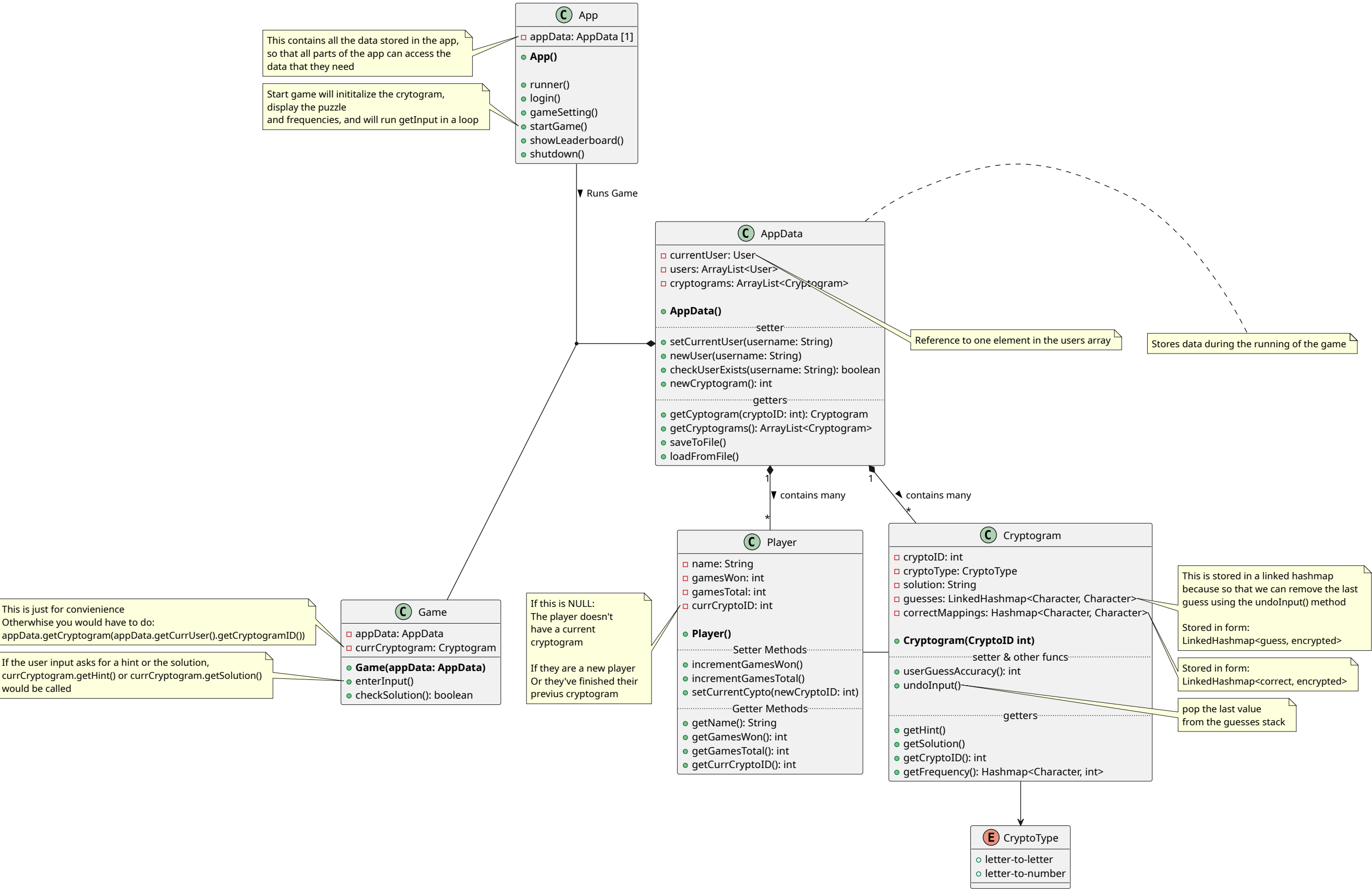
CS207 Cryptogram Project - Class Diagram - Group 25 2026
