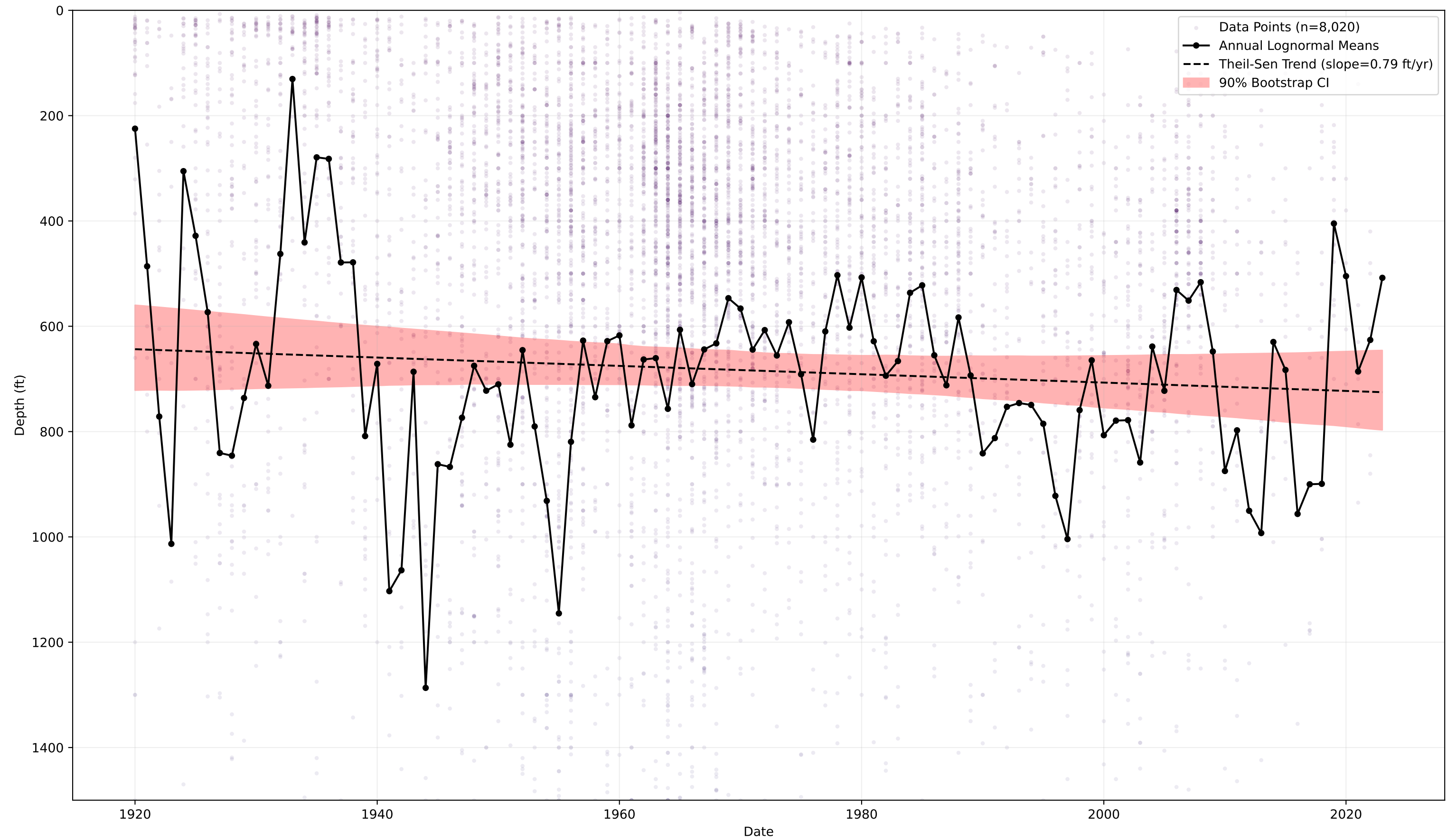
Carrizo-Wilcox Aquifer Depth Analysis: 1920-2023 Theil-Sen Trend with 90% Bootstrap CI
