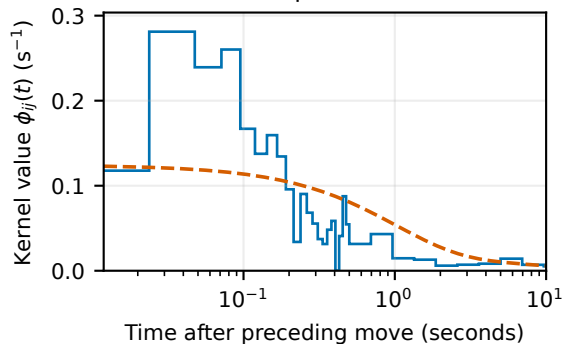
(c) Bid up \rightarrow Bid down
