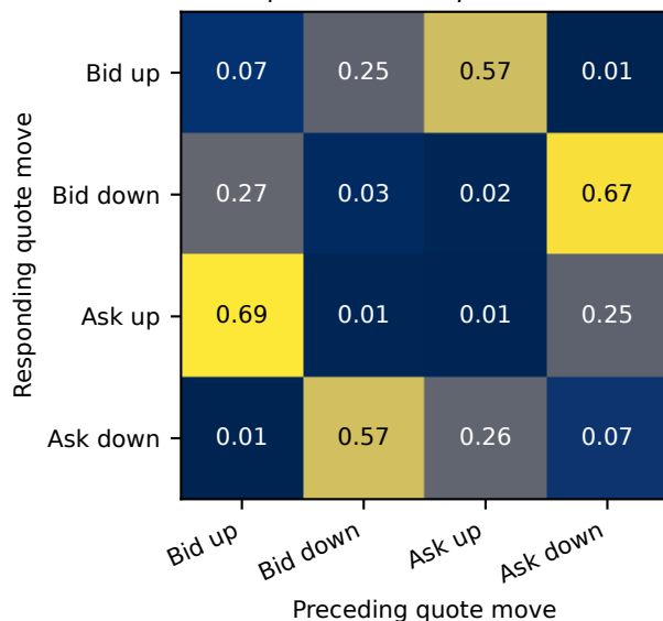
(b) Converged EM fit Spectral radius \rho = 0.9373
