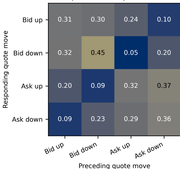
(a) Conditional least squares Spectral radius \rho = 0.9784
