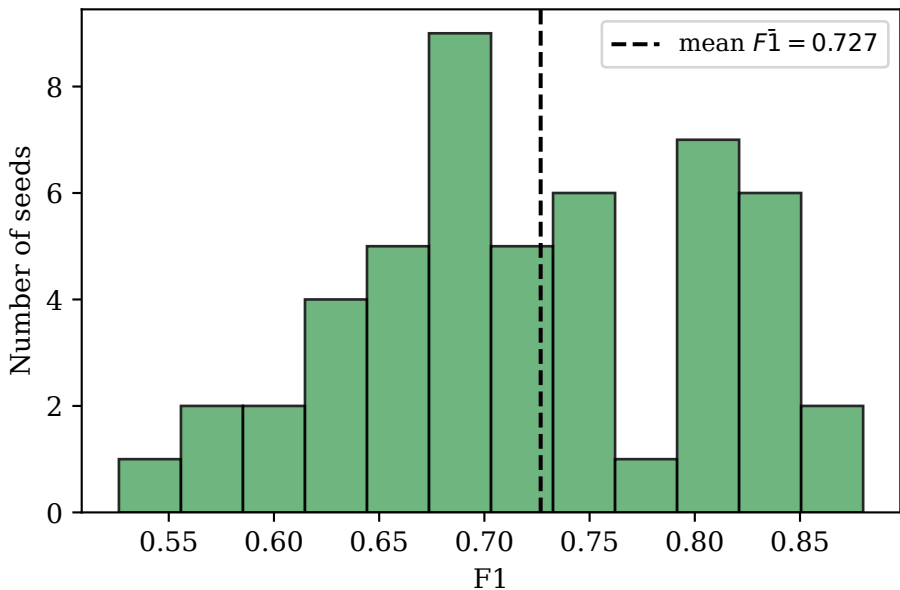
Per-seed F1 on the meta-order smoke benchmark, 50 seeds \bar{F1} = 0.727 , \sigma = 0.083
