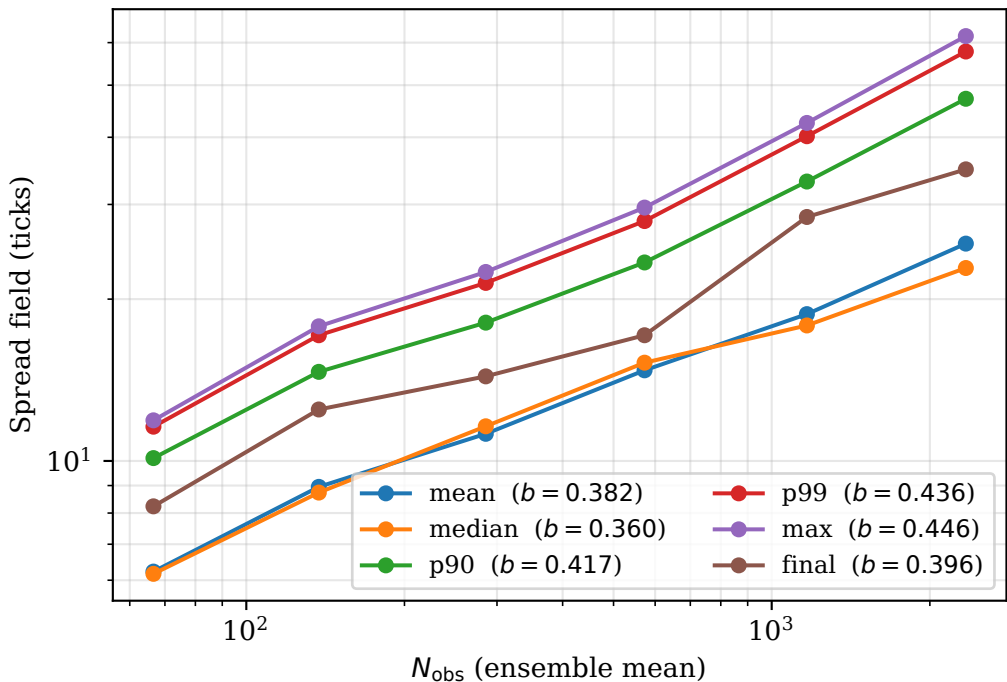
Spread-scaling diagnostic on the first-milestone configuration (30 seeds per horizon; T \in \{30, 60, 120, 240, 480, 960\} )
