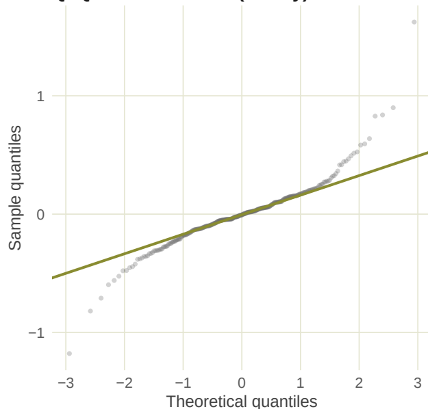
Q-Q: random effects (colony)
