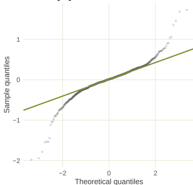
Normal Q-Q – residuals
