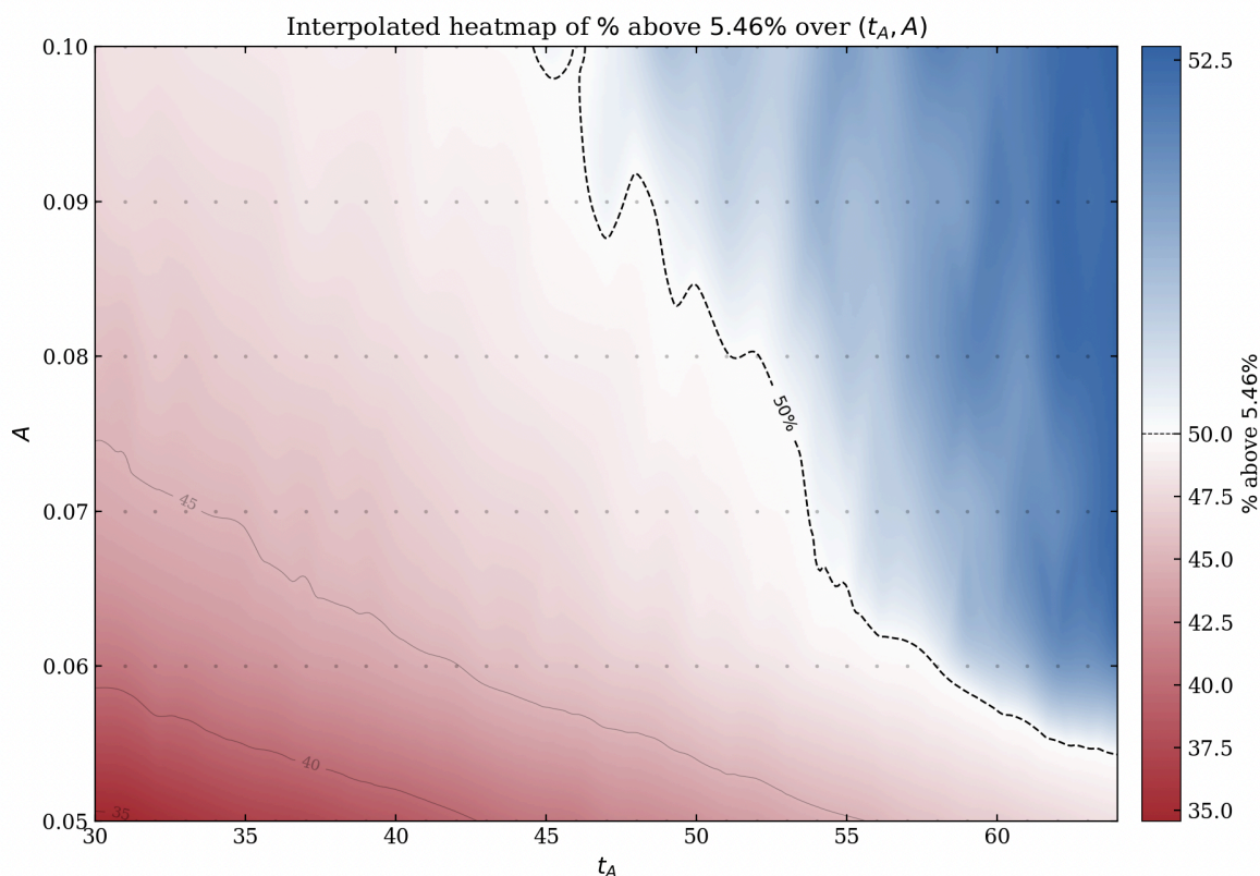
[FIGURE 3: Heatmap of success probability \Psi over the (A, T_A) grid at R^* = UF + 5.5\% . The 50% contour separates successful from unsuccessful curves.]
