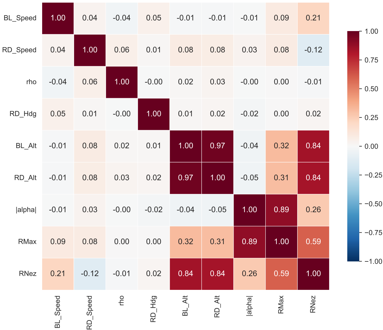
Spearman correlation — feasible Random/WEZ subset ( n = 964 )
