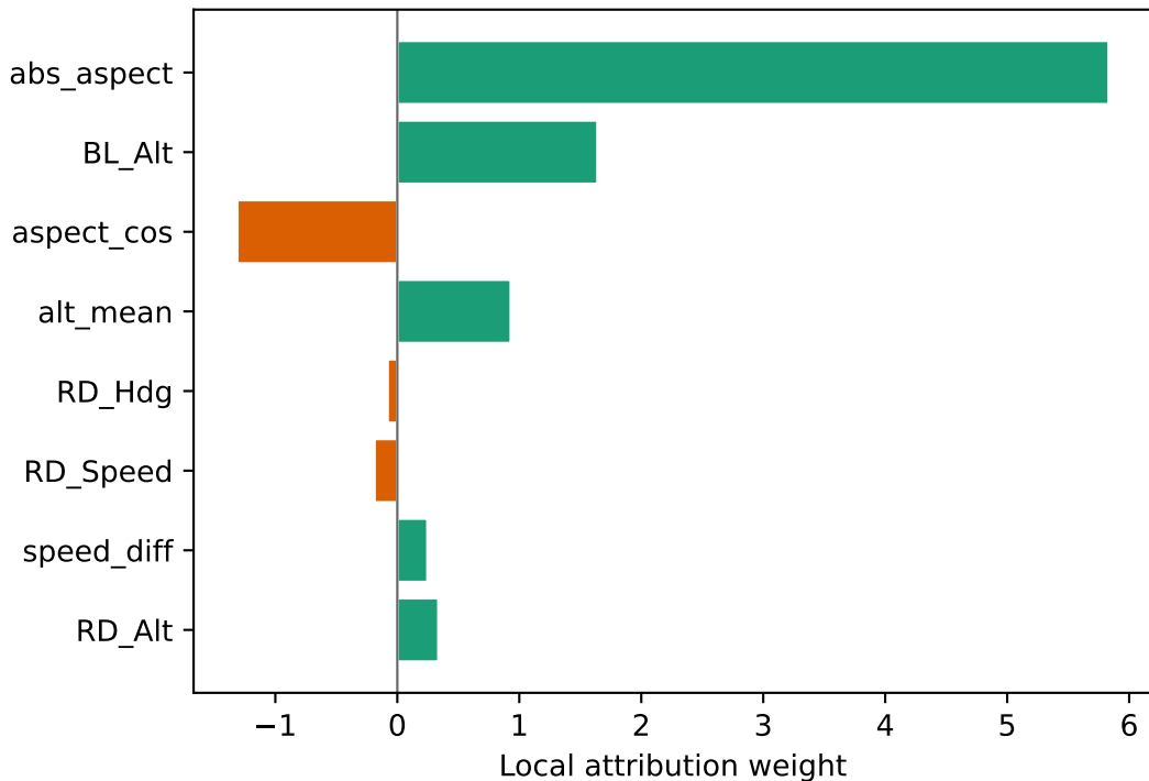
LIME (local linear surrogate)
