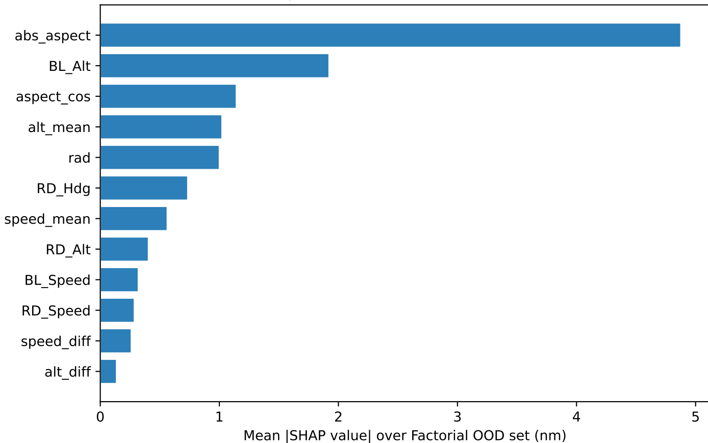
Global feature importance via TreeSHAP — XGBoost+Monotone
