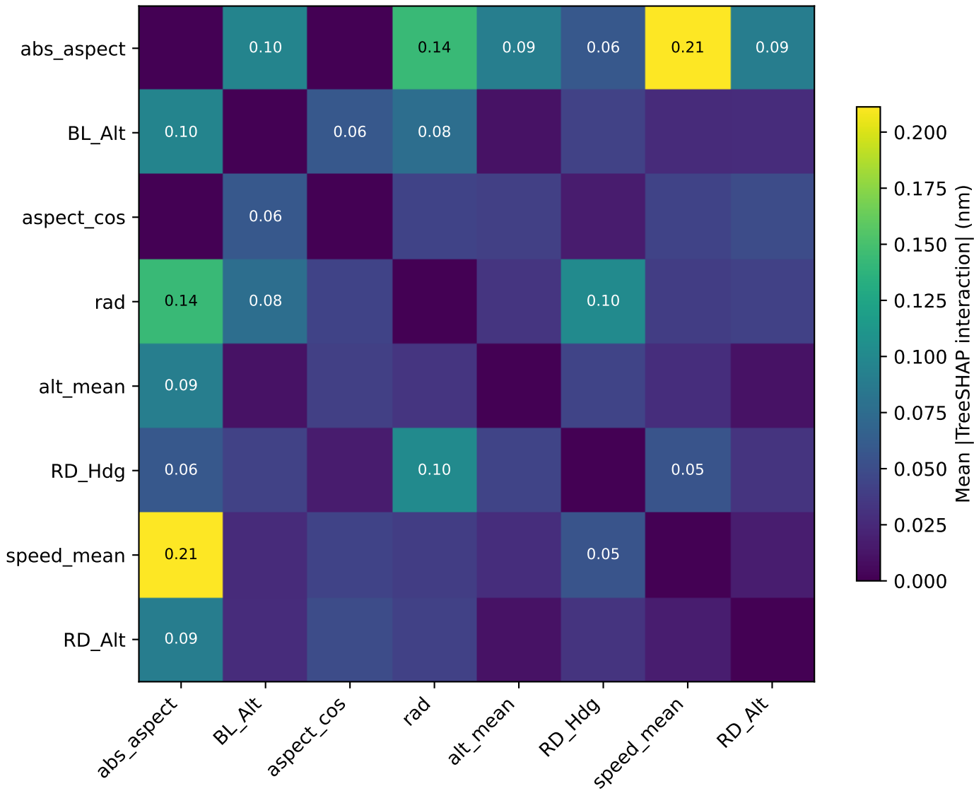
Pairwise TreeSHAP interactions (off-diagonal) — top-8 features
