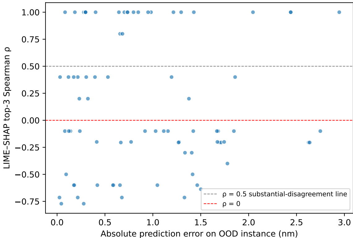
Disagreement vs prediction error (N=80, XGB+Monotone)
