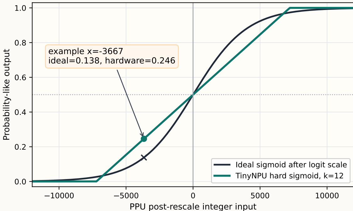
Calibrated fused hard-sigmoid response
