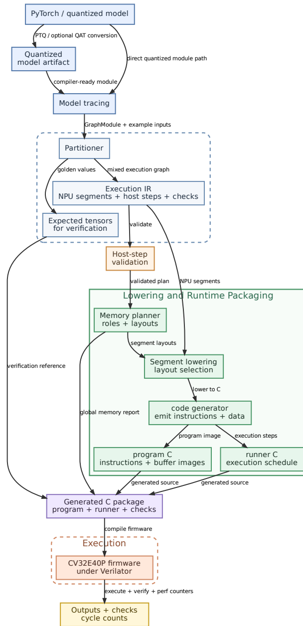
Figure 3.4: Compiler and firmware flow used to execute a TinyNPU artifact.
