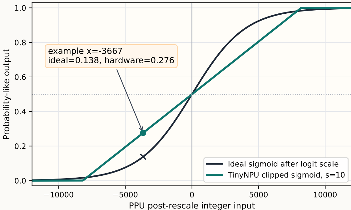
Calibrated fused sigmoid response
