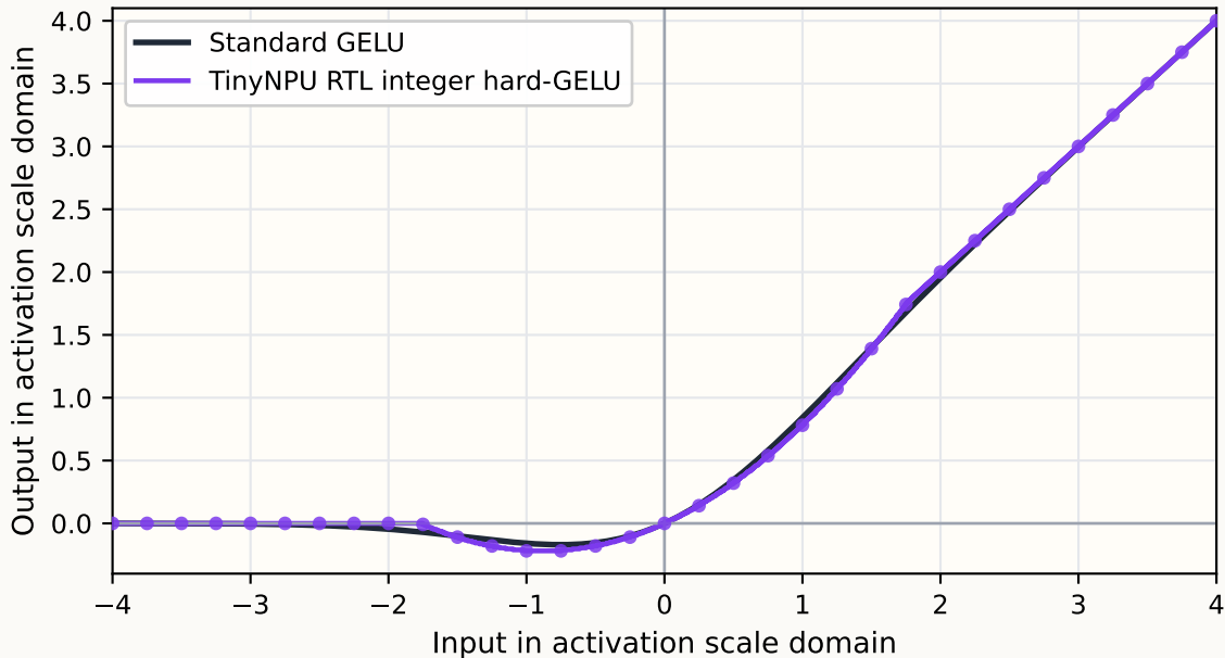
Hard-GELU integer response
