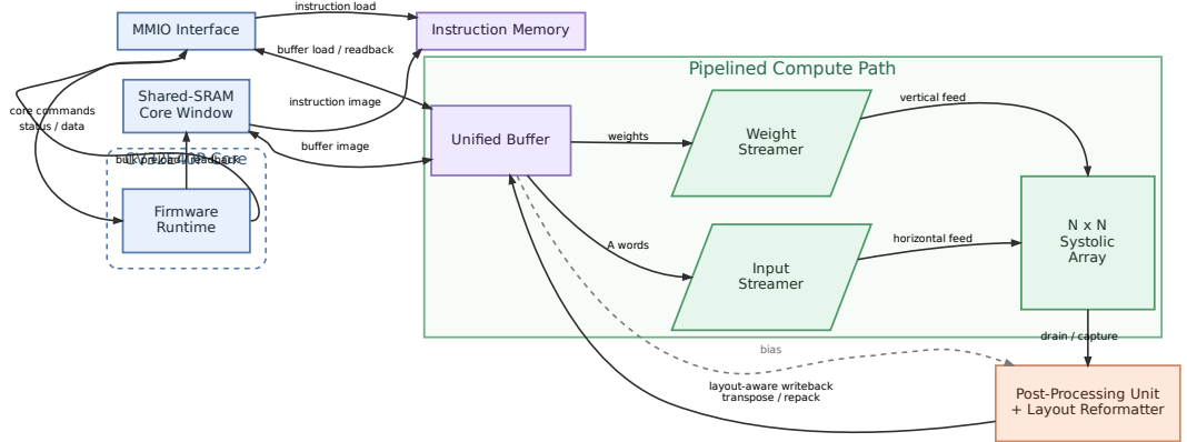
Figure 3.1: Top-level TinyNPU hardware architecture.
