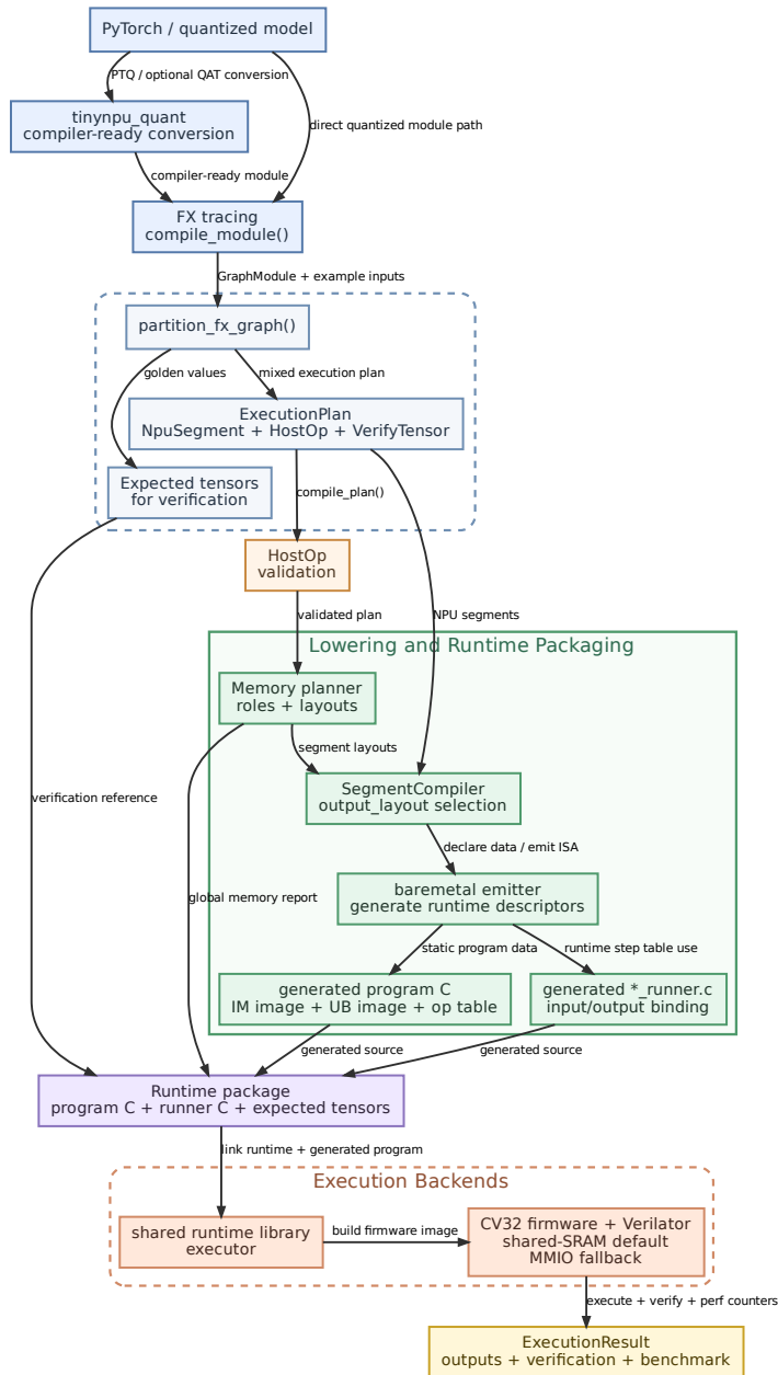
Figure 3.4: Compiler and runtime flow used by the TinyNPU JIT path.
