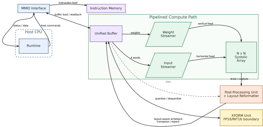
Figure 3.1: Top-level TinyNPU hardware architecture.
