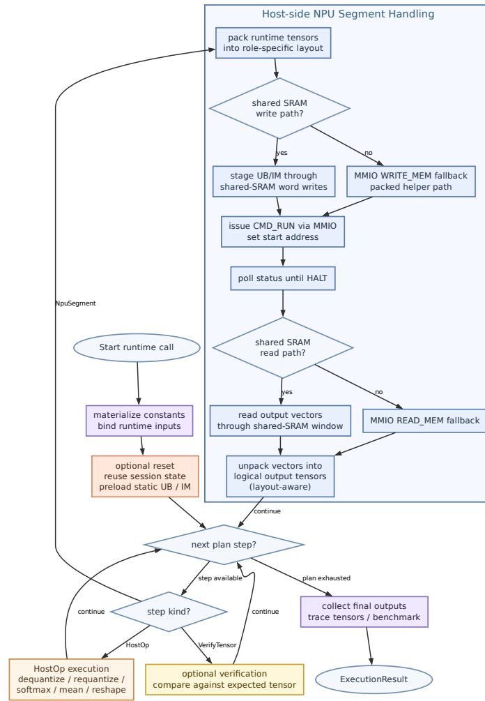
Figure 3.5: Host-side runtime flow for executing a compiled TinyNPU artifact.
