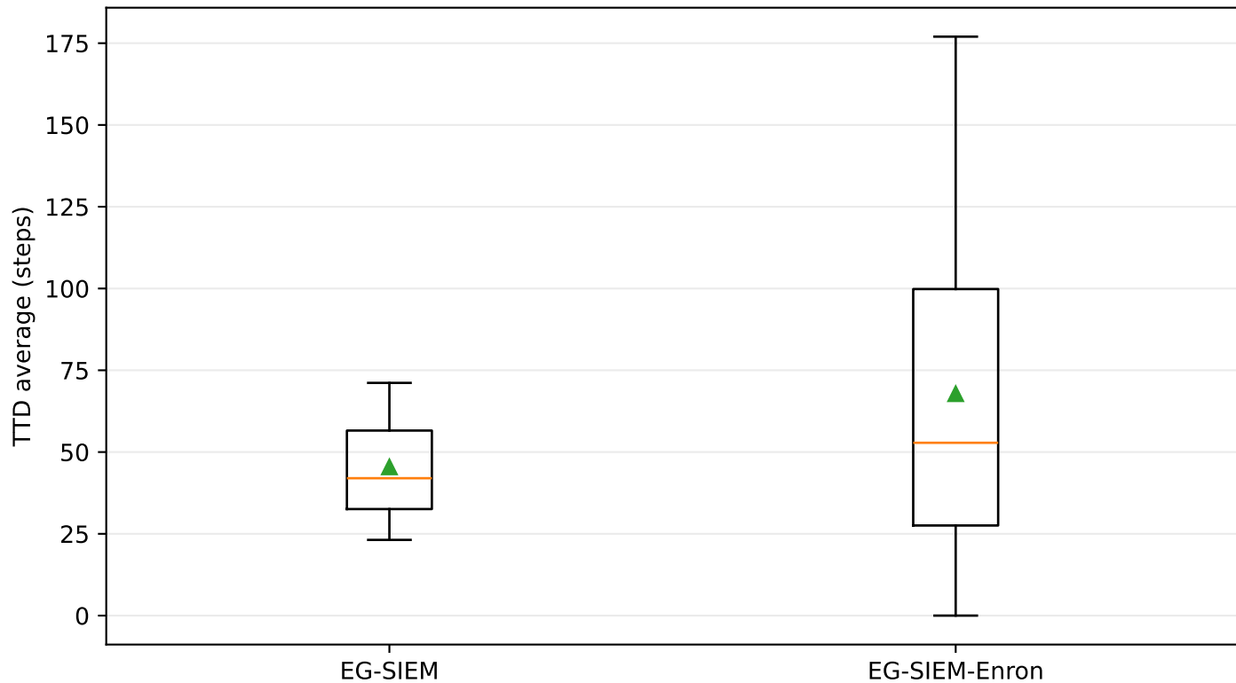
TTD average (steps) by variant
