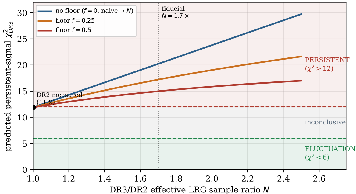
Pre-registered DR3 test: systematic floor caps the growth
