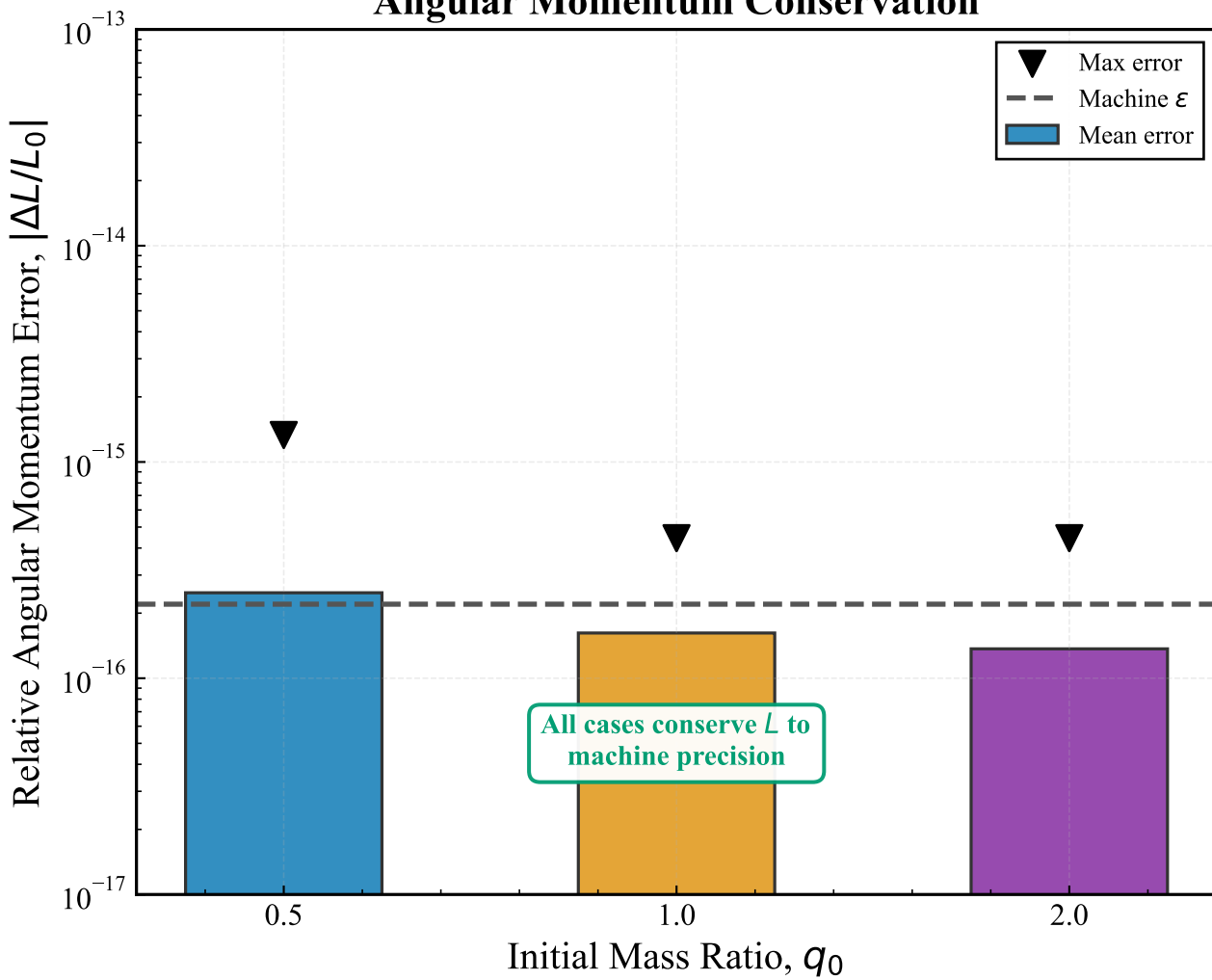
Angular Momentum Conservation
