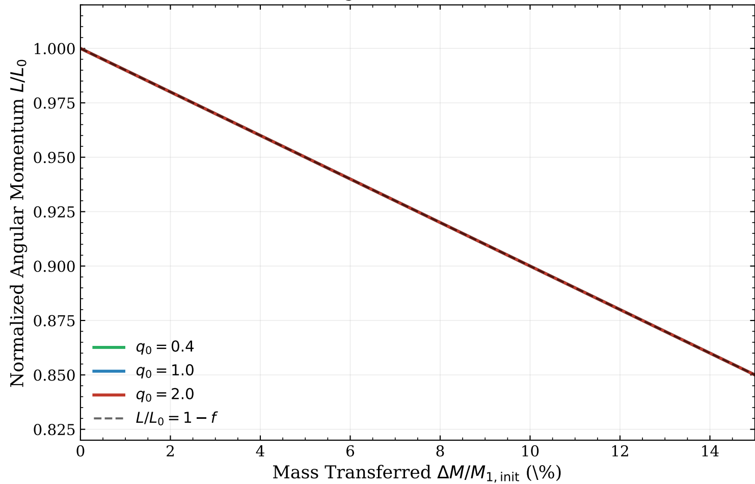
(a) Angular Momentum Loss
