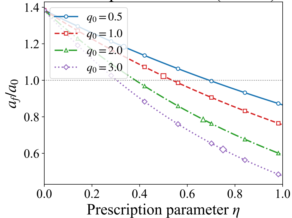
Final separation ratio (f=0.15)
