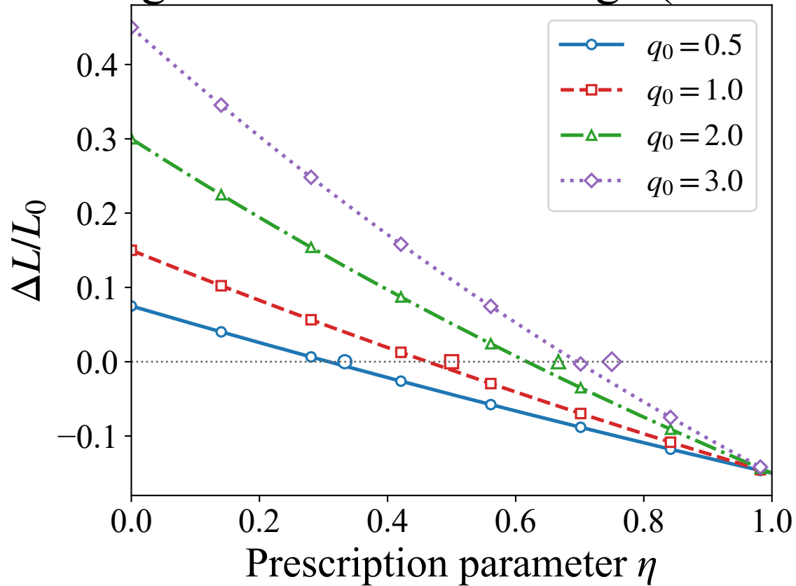
Angular momentum change (f=0.15)
