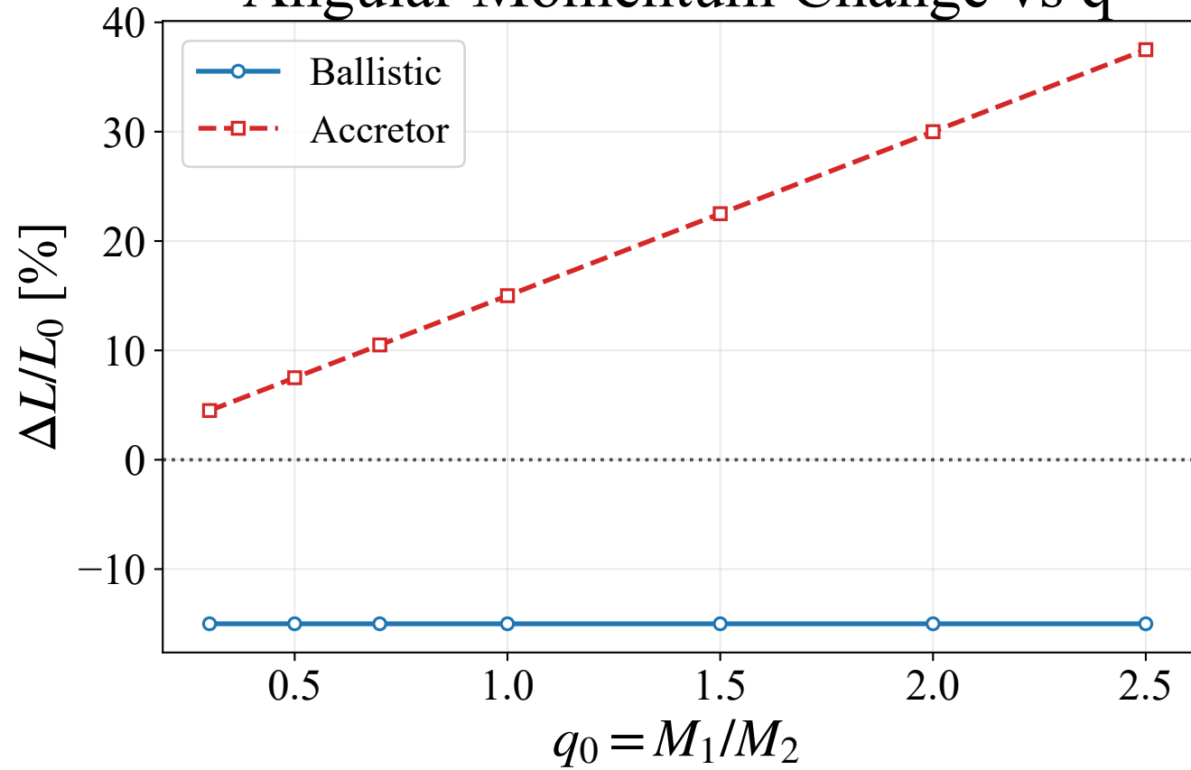
Angular Momentum Change vs q
