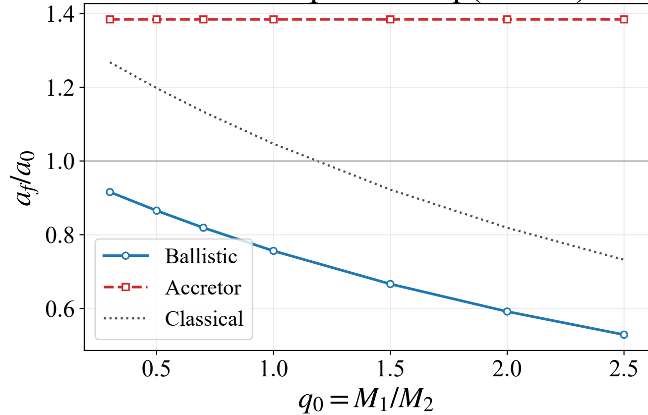
Orbital Response vs q ( f=0.15 )
