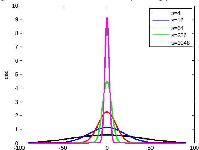
Figure 4.2 Effects of a variation in s for the directional spreading of wave energy. The x-axis shows degrees, the y-axis the distribution where the integral under the curves is unity.
