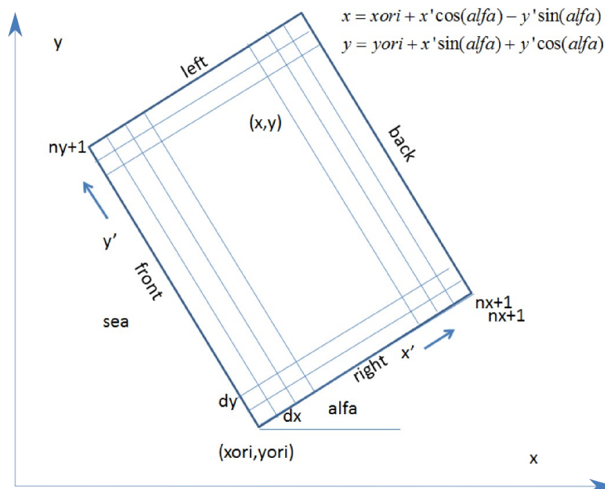
Figure 212Equation Chapter 2 Section 1Processes and model formulation.1 Rectangular coordinate system of XBeach, with world coordinates ( x , y ) and model coordinates ( x' , y' ).
