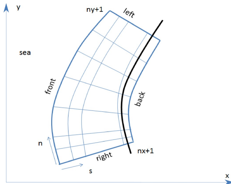
Figure 212Equation Chapter 2 Section 1Processes and model formulation.2 Curvilinear coordinate system of XBeach
