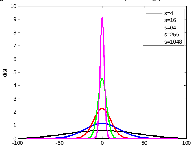
Figure Input description.14 Effects of a variation in s for the directional spreading of wave energy. The x-axis shows degrees, the y-axis the distribution where the integral under the curves is unity.
