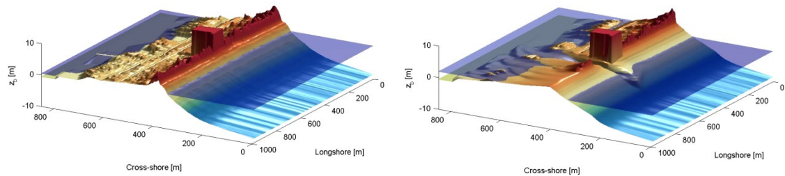
Figure 212 Equation Chapter 2 Section 1 Processes and model formulation.6 Pre (left) and post-Sandy (right) in a three dimensional plot with both bed and water levels as simulated by XBeach (Nederhoff et al. 2015)
