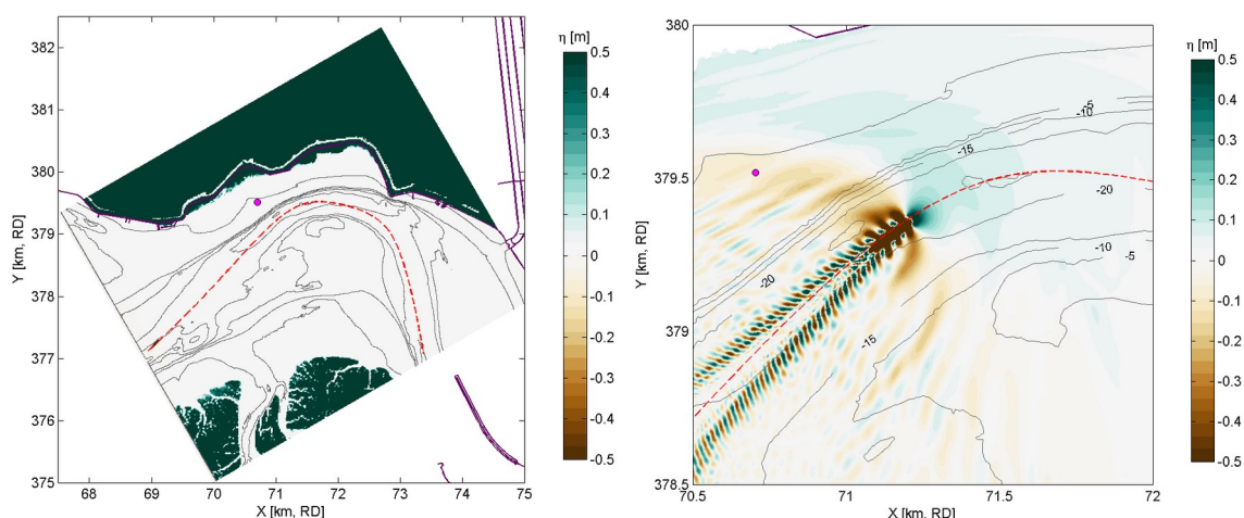
Figure 212Equation Chapter 2 Section 1Processes and model formulation.9 Example XBeach setup (left) and result (right) for a ship wave simulation in the Scheldt Estuary (The Netherlands). The ship track (red dashed line) is user-defined, and the measurement location is indicated (magenta dot).
