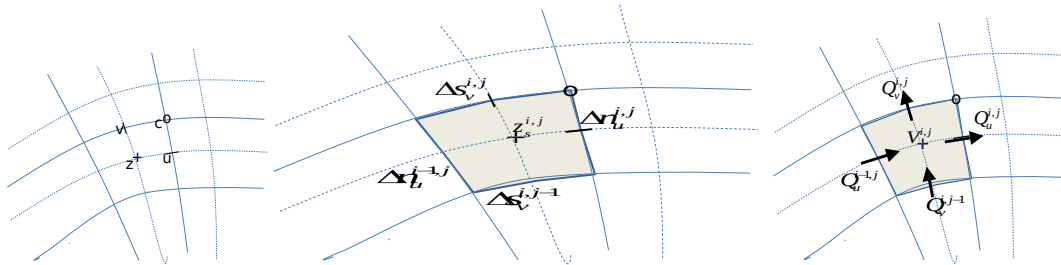
Figure References.17 Location of staggered grid points (left panel); definition of grid distances (middle) and terms in volume balance (right)
