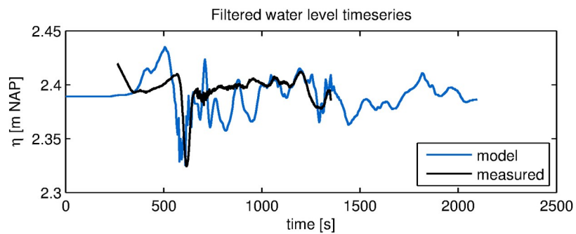
Figure 212Equation Chapter 2 Section 1Processes and model formulation.10 Example XBeach result for ship-induced waves. Measurements are taken at Bath, in the Scheldt Estuary, The Netherlands (Schroevens et al., 2011).
