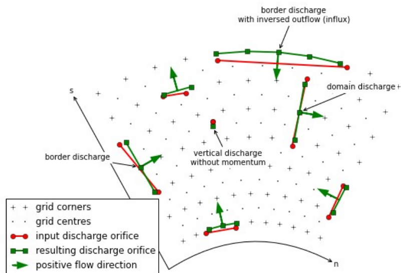
Figure Input description.16 Possible discharge orifices. A discharge orifice is defined as line in between two points (red). The resulting discharge orifice constitutes out of full abreast grid cells (green). The discharge direction is in positive grid direction (s or n), except at the domain border where the discharge is an influx in the domain (green arrows).
