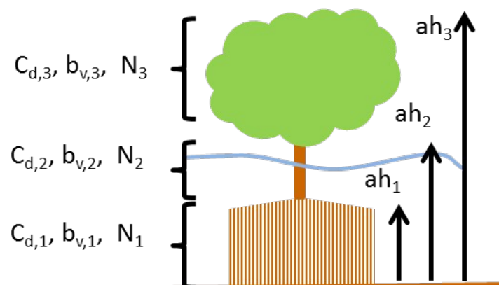
Figure Input description.15 Definition sketch of vegetation specification in XBeach (example for mangrove type vegetation schematized in three vertical sections).
