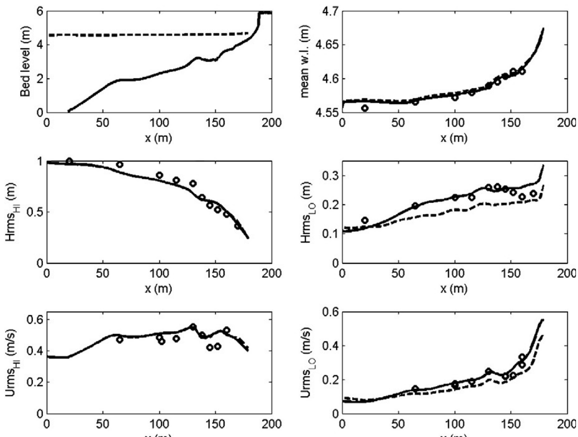
Figure 212Equation Chapter 2 Section 1Processes and model formulation.5 Computed and observed hydrodynamic parameters for test 2E of the LIP11D experiment (2E). Top left: bed level and mean water level. From top to bottom: measured (dots) and computed mean water levels, wave heights for the low en high frequency bands ( H_{rms} ) and velocities for the high and low frequency bands ( u_{rms} ).
