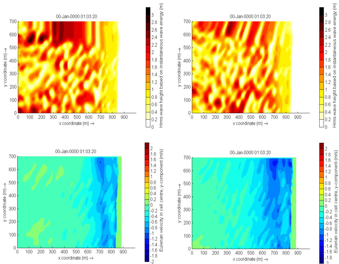
Figure Boundary conditions.11 Effect of the lateral wave boundary conditions on root-mean square wave height patterns (top) and longshore velocity (bottom) for the Delilah test case. In this figure the left panels are used for simulations with Neumann boundaries and the right panel with the wavecrest boundary.
