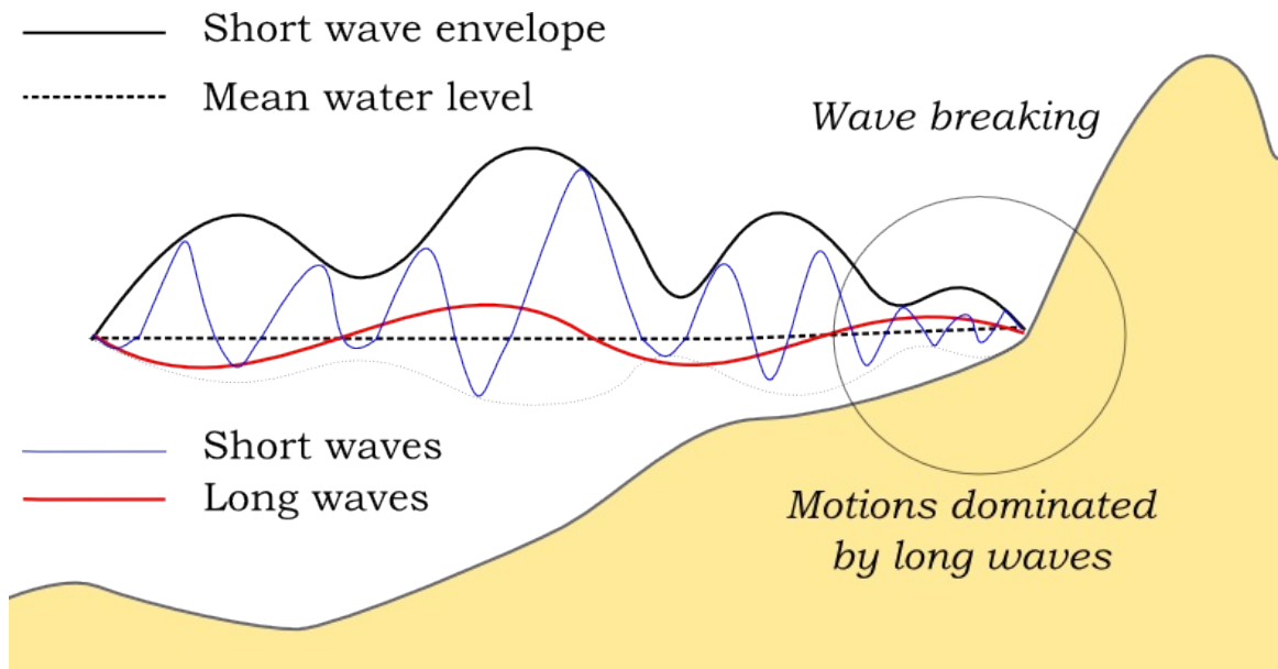
Figure 212 Equation Chapter 2 Section 1 Processes and model formulation.3 Principle sketch of the relevant wave processes
