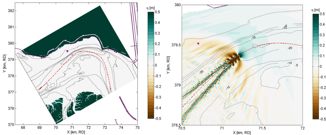
Figure 2.10 Example XBeach setup (left) and result (right) for a ship wave simulation in the Scheldt Estuary (The Netherlands). The ship track (red dashed line) is user-defined, and the measurement location is indicated (magenta dot).
