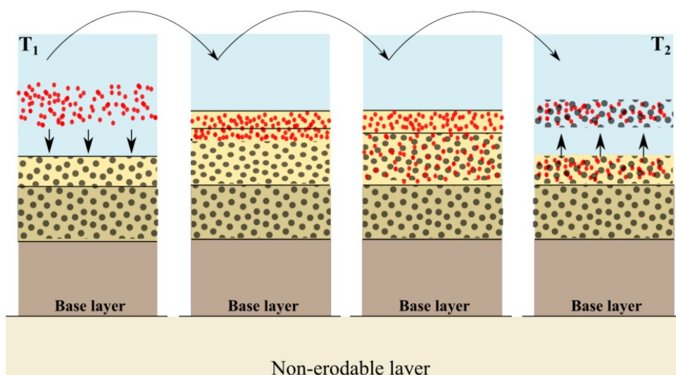
Figure 2.9 Visualization of the diffusion that occurs when XBeach calculates sediment compositions. After sedimentation of fine sediment on top of coarser material it is uniformly mixed over the whole layer.
