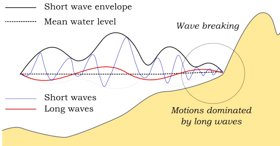
Figure Processes and model formulation.3 Principle sketch of the relevant wave processes
