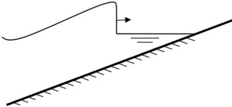
Figure Processes and model formulation.8 During wave breaking and wave runup the wave is modelled as a bore (Smit et al, 2010)
