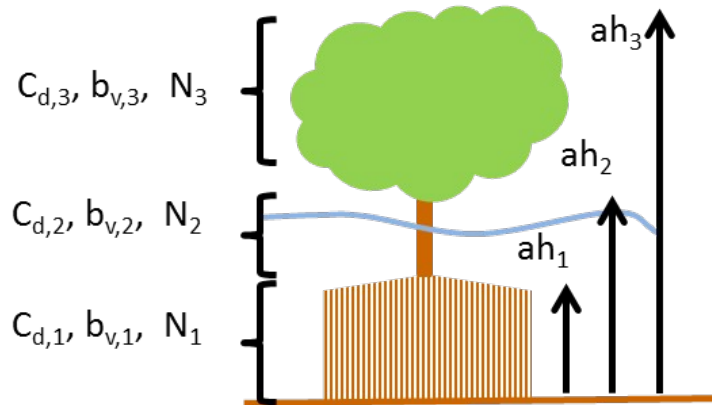
Figure Input description.16 Definition sketch of vegetation specification in XBeach (example for mangrove type vegetation schematized in three vertical sections).
