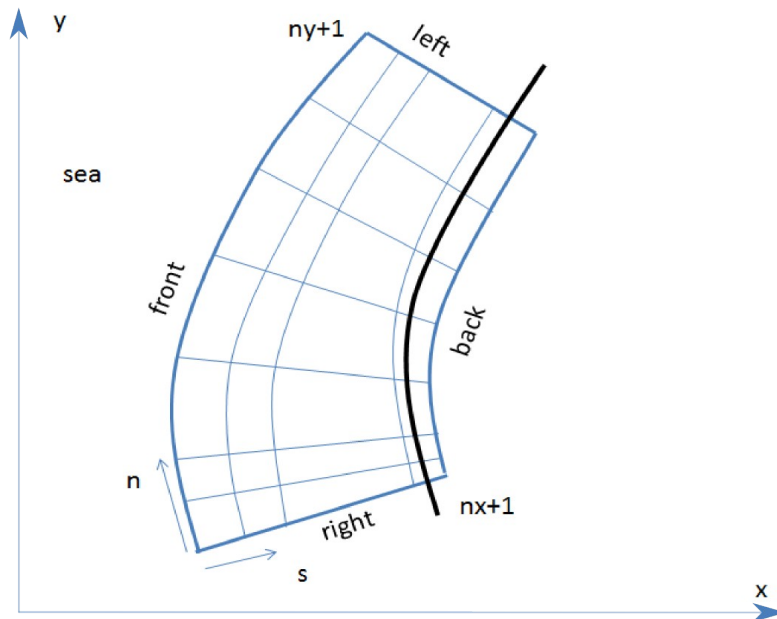
Figure Processes and model formulation.2 Curvilinear coordinate system of XBeach
