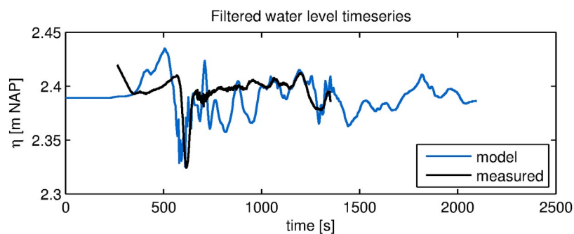
Figure Processes and model formulation.11 Example XBeach result for ship-induced waves. Measurements are taken at Bath, in the Scheldt Estuary, The Netherlands (Schroevens et al., 2011).
