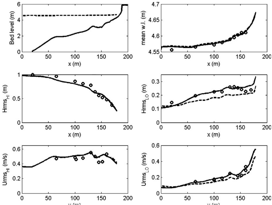
Figure Processes and model formulation.5 Computed and observed hydrodynamic parameters for test 2E of the LIP11D experiment. Top left: bed level and mean water level. Top right: measured (dots) and computed
