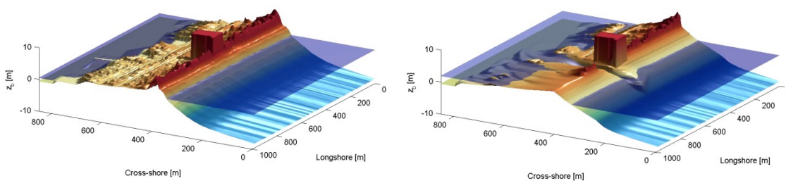
Figure Processes and model formulation.6 Pre (left) and post-Sandy (right) in a three dimensional plot with both bed and water levels as simulated by XBeach (Nederhoff et al. 2015)
