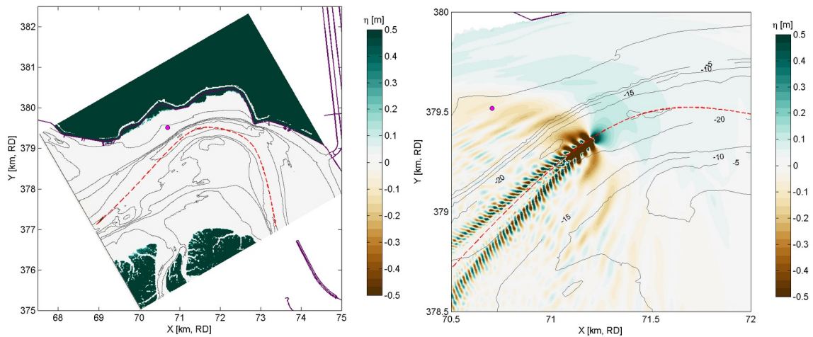
Figure Processes and model formulation.10 Example XBeach setup (left) and result (right) for a ship wave simulation in the Scheldt Estuary (The Netherlands). The ship track (red dashed line) is user-defined, and the measurement location is indicated (magenta dot).
