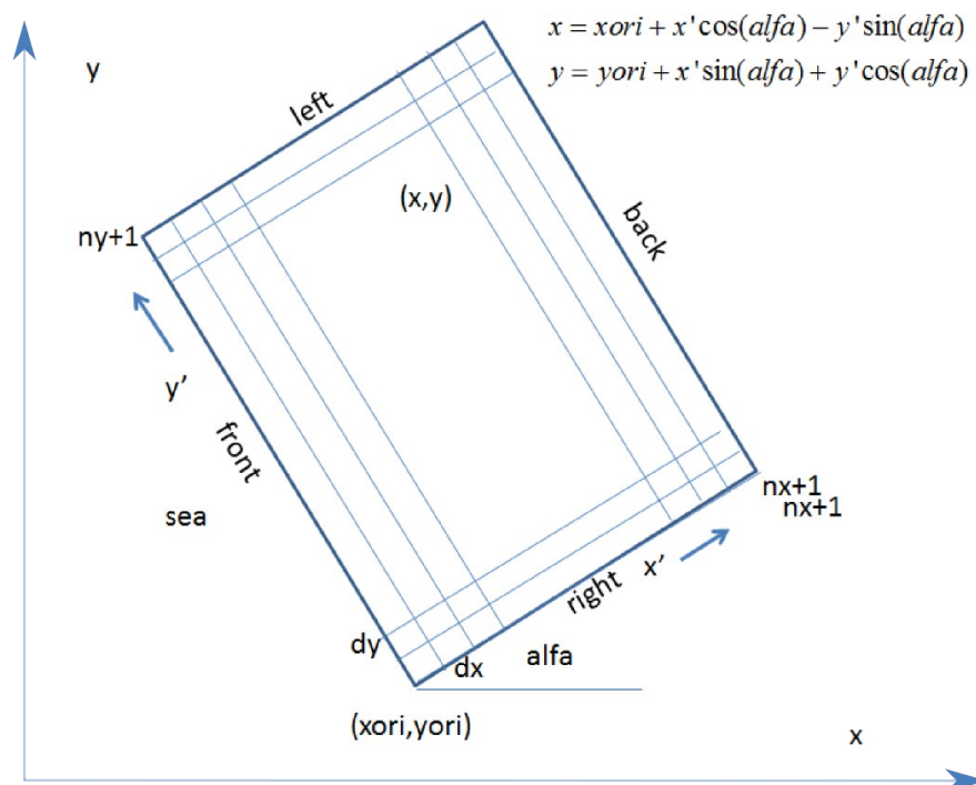
Figure Processes and model formulation.1 Rectangular coordinate system of XBeach
