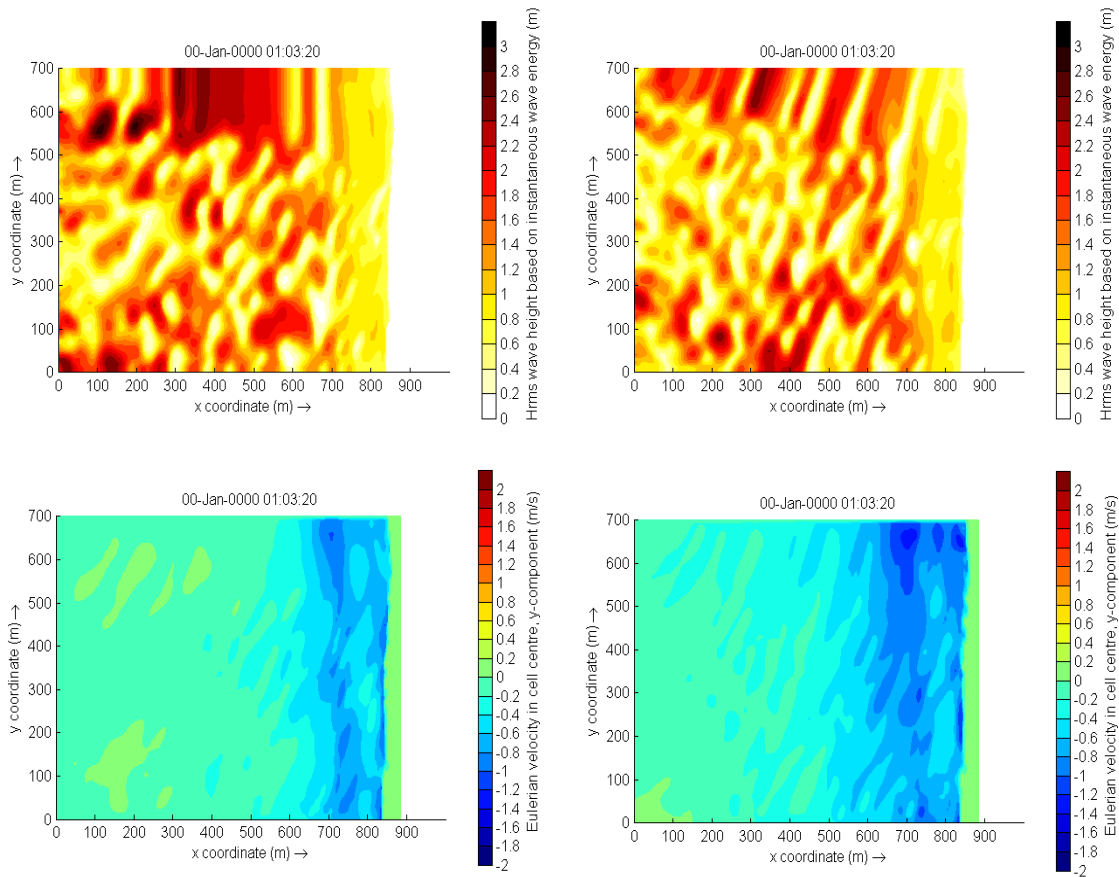
Figure Boundary conditions.12 Effect of the lateral wave boundary conditions on root-mean square wave height patterns (top) and longshore velocity (bottom) for the Delilah test case. In this figure the left panels are used for simulations with Neumann boundaries and the right panel with the wavecrest boundary.
