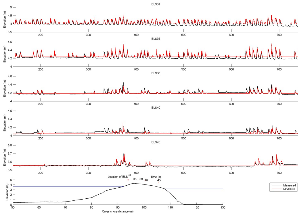
Figure Processes and model formulation.7 Measured (black) and modeled (red) time series of overtopping during BARDEX experiment, from McCall et al, 2014.
