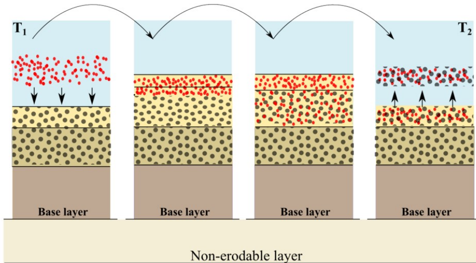
Figure Processes and model formulation.9 Visualization of the diffusion that occurs when XBeach calculates sediment compositions. After sedimentation of fine sediment on top of coarser material it is uniformly mixed over the whole layer. Subsequent erosion erodes both the fines as the coarser material. To avoid this phenomenon, layers should not be too thick (van der Zwaag, 2014).
