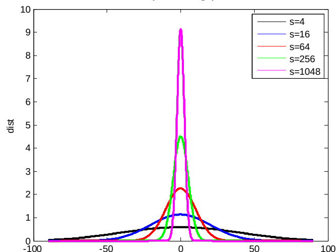
Figure Input description.15 Effect a variation in s for the direction spreading of wave energy
