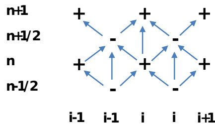
Leap-frog time integration scheme
