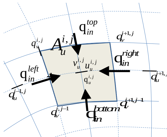
Control volume u-momentum balance and definition of fluxes
