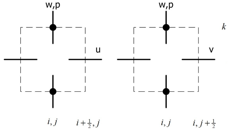
Figure Numerical model-5 Vertical location of variables.
