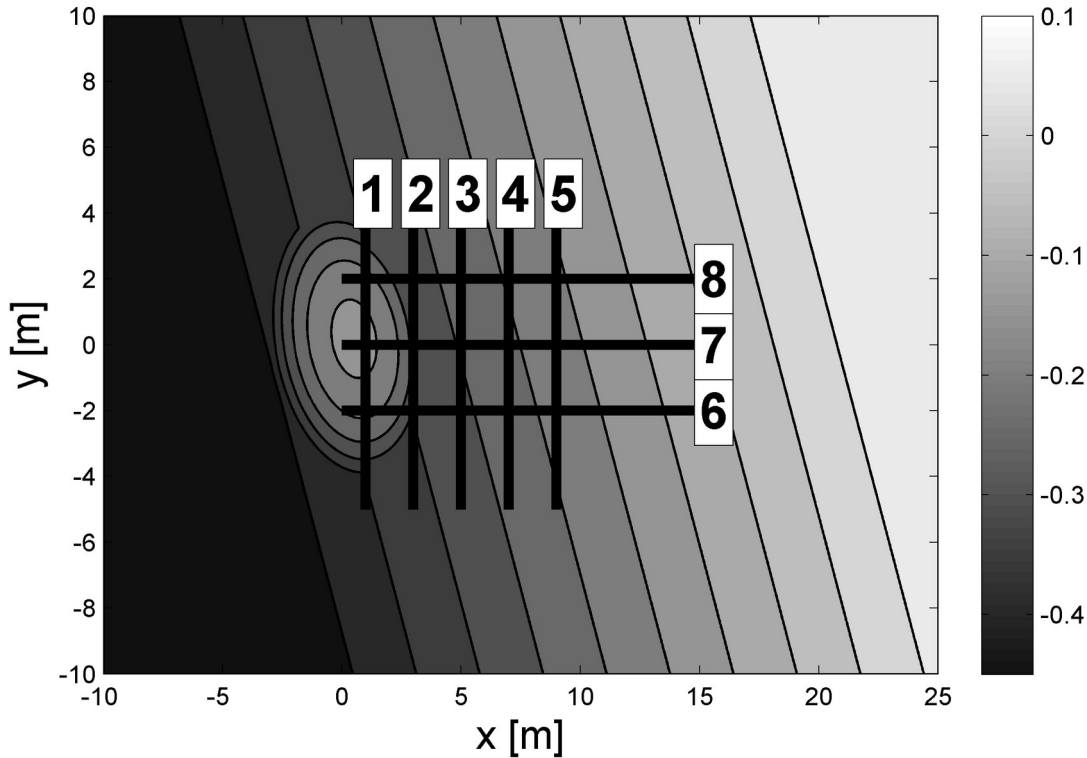
Figure Verification and validation-21 Bathymetry of the experiment carried out by Berkhoff et. al. and the location of the transects along which measurements were conducted.
