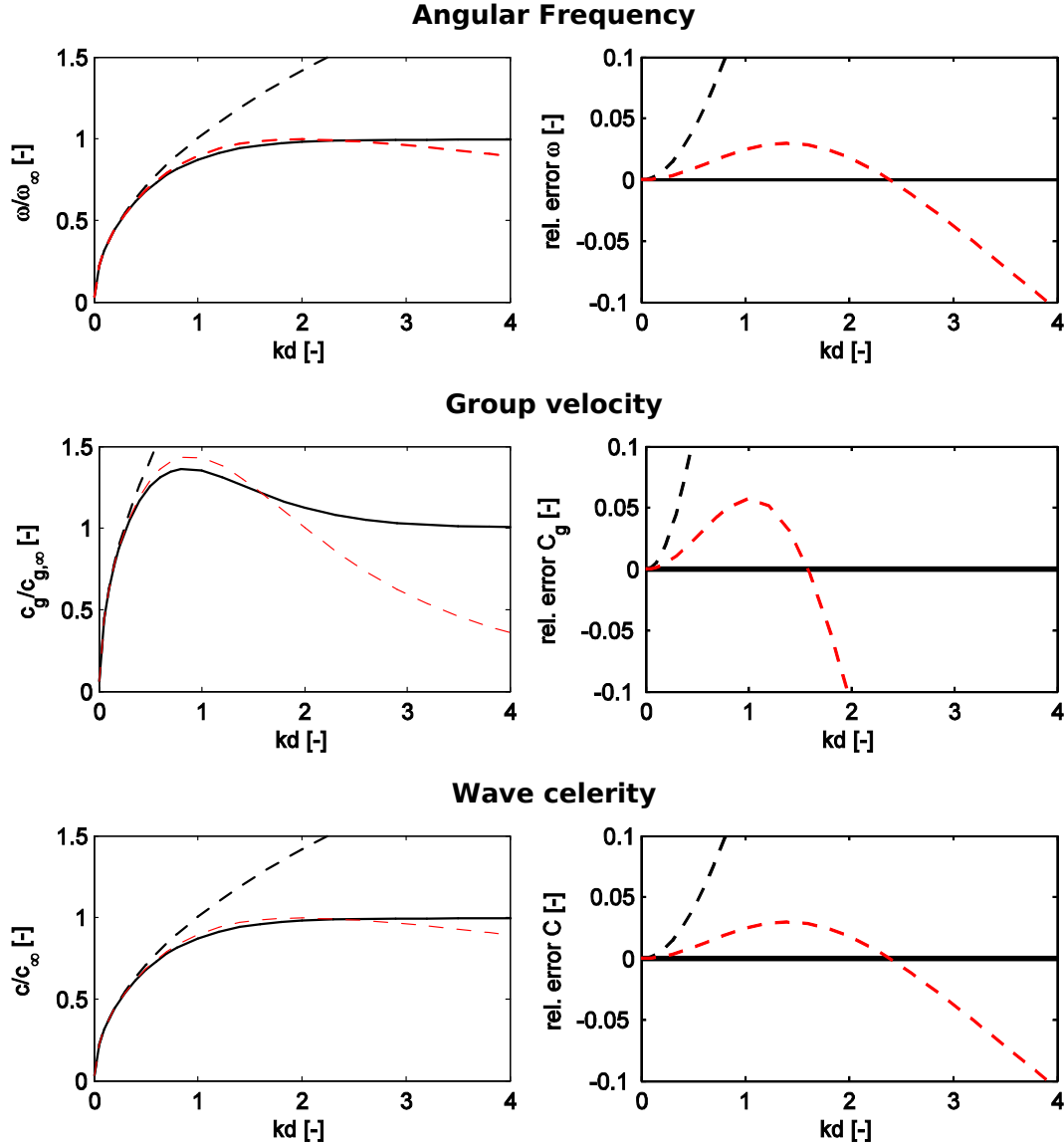
Figure Verification and validation-9 The angular frequency, group velocity and wave celerity for a constant wave length in varying depth. Computed from linear wave theory (black line), the shallow water approximation (dotted black line) and the semi discrete relations (dotted red line). The left hand panels give the values scaled with their respective deep water values, while the right hand panels show the relative errors compared to linear wave theory.
