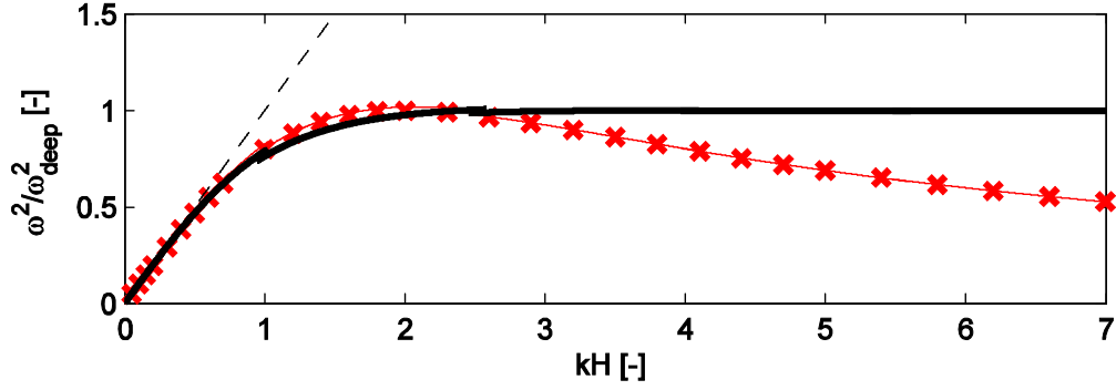
Figure Verification and validation-12 The dispersion relation for a wave with constant wavelength in varying depth. Shown are the linear dispersion relation (thick black line), semi-discrete dispersion relation (red line), model results (red crosses) and the shallow water dispersion relation (striped black line).
