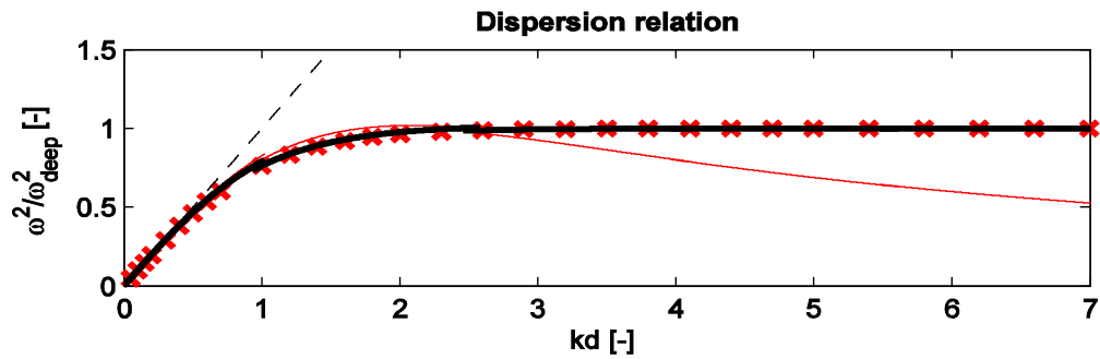
Figure Verification and validation-14 Linear dispersion relation (thick black) line compared to the numerical dispersion relation (red line) and the numerical dispersion relation with optimized coefficients (red crosses).
