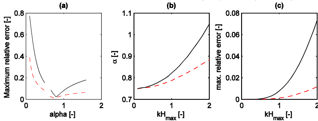
Figure Verification and validation-15 (a) The maximum relative error in the range 0 < kH < 1 as a function of \alpha for c_g (black) and \omega (red). (b) The optimum value of \alpha minimizing the maximum relative error over the range 0 < kH < kH_{max} . Optimum value for c_g (black) and \omega (red) (c) The maximum relative error at the optimum value of \alpha over the range 0 < kH < kH_{max} . Error indicated for c_g (black) and \omega (red).
