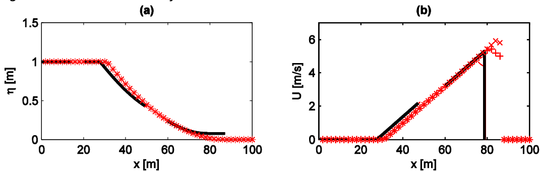
Figure Verification and validation-19 Dry dambreak case. (a) free surface elevation for the analytical solution (thick black line), the first order scheme (red plusses) and the second order scheme (red crosses). (b) horizontal velocity for the analytical solution (thick black line), the first order scheme (red plusses) and the second order scheme (red crosses).
