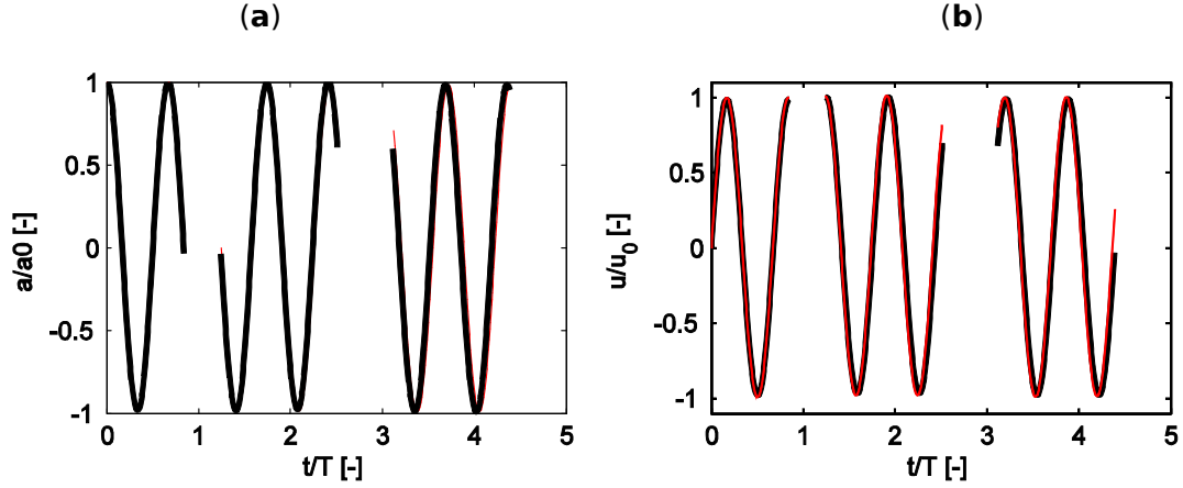
Figure Verification and validation-10 (a) Free surface elevation at (1,1) scaled with the amplitude. Analytical solution (black) compared to the numerical solution (red). (b) Horizontal velocity scaled with the velocity amplitude. Analytical solution (black) compared to the numerical solution (red).
