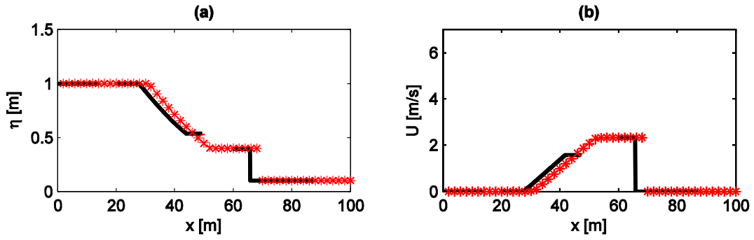
Figure Verification and validation-20 Wet dam-break case. (a) free surface elevation for the analytical solution (thick black line), the first order scheme (red plusses) and the second order scheme (red crosses). (b) horizontal velocity for the analytical solution (thick black line), the first order scheme (red plusses) and the second order scheme (red crosses).
