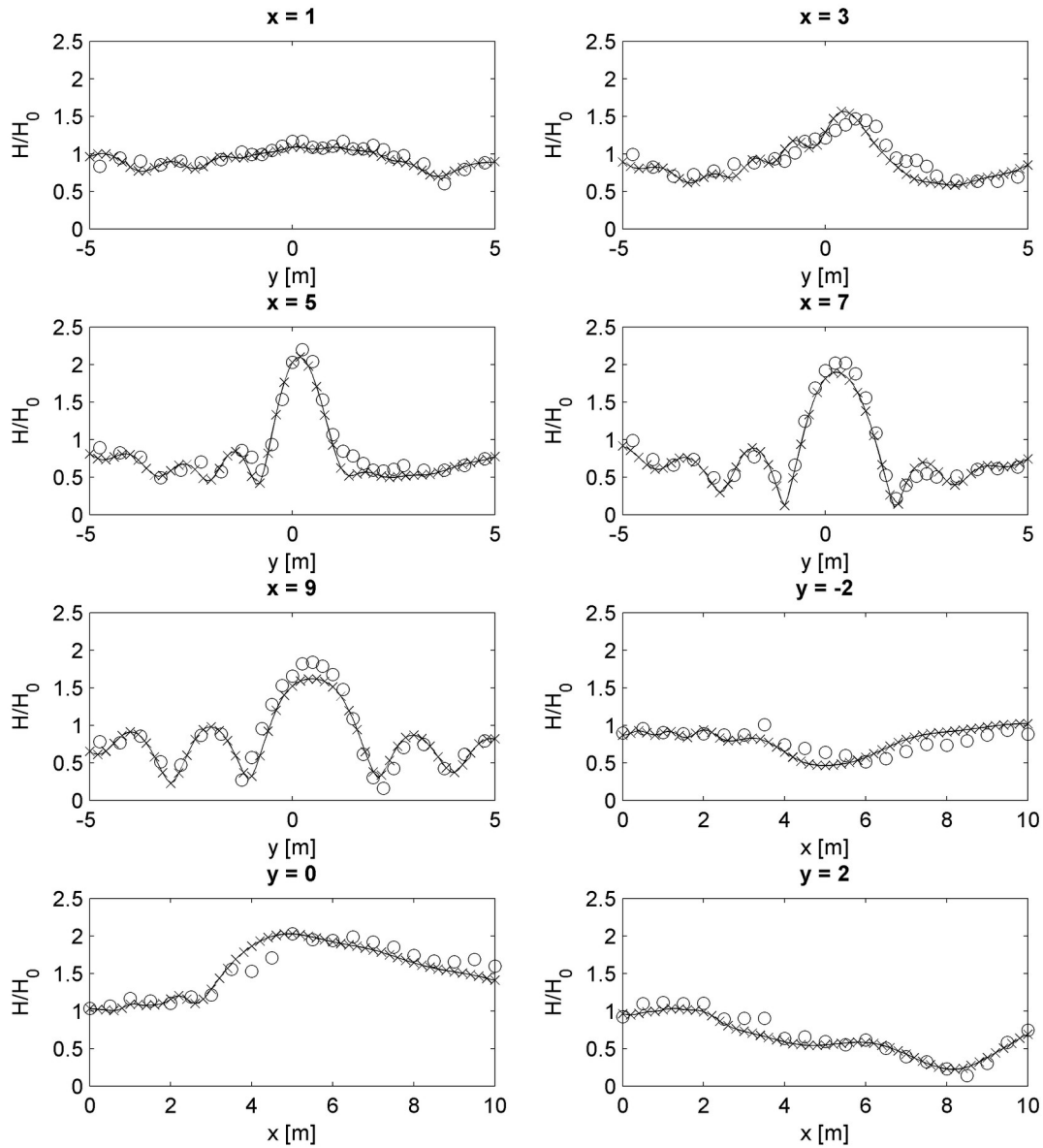
Figure Verification and validation-22 The relative wave height along the eight transects. Measurements are indicated with circles while .Comparison between measurements (symbols) and the results using a depth averaged approach. Shown are the relative wave heights along the eight transects (waves scaled with the incoming wave height).
