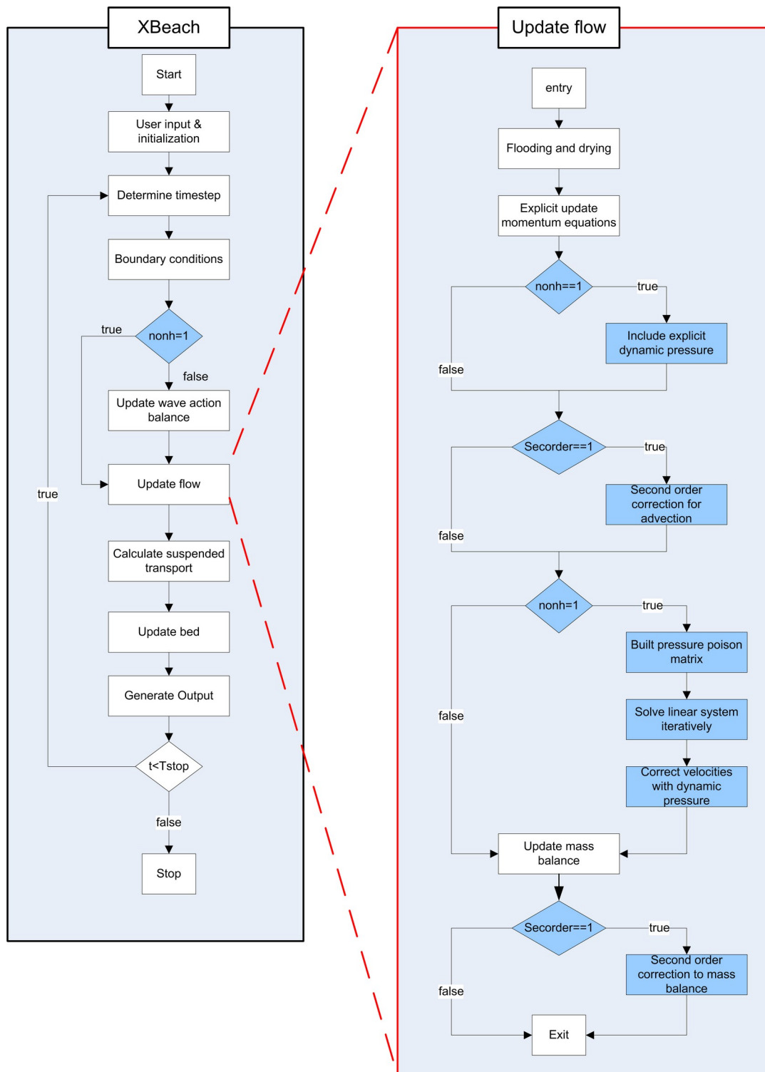
Figure Implementation and usage-23 Flowchart showing the structure of the main program on the left and a detailed overview of the flow module on the right. Note that processes already described in XBeach are denoted as white boxes while new processes are in blue.
