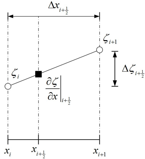
Figure Numerical model-7 For non-uniform grids central approximation reduce locally to first order accuracy
