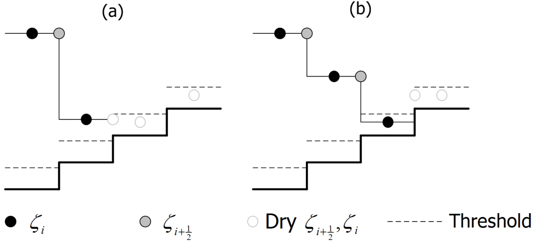
Figure Numerical model-8 (a) A velocity point is considered dry if the total water depth is under a certain threshold. (b) A water level point is considered wet if any of the surrounding velocity points are wet, even if the water depth itself is below the threshold.
