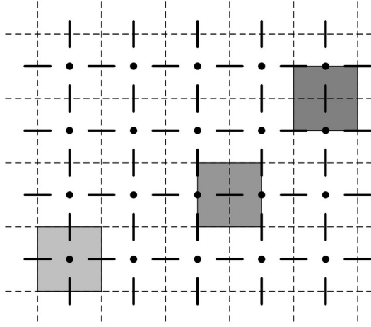
Figure Numerical model-4 Horizontal location of variables.
