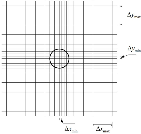
Figure Numerical model-6 Example of a non-uniform structured grid
