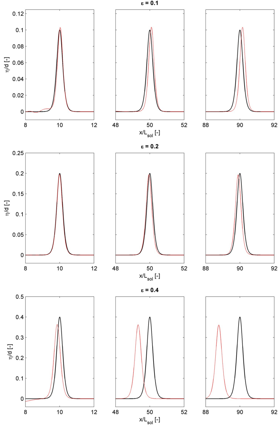
Figure Verification and validation-17 The free surface elevation of a solitary wave propagating through a channel of uniform depth. Model (red) and analytical (black) results for three different incident waves shown at three different locations in the channel.
