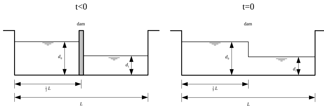
Figure Verification and validation-18 Dam break case. Two reservoirs are separated by a structure (left), but at t=0 suddenly the structure is removed (right).
