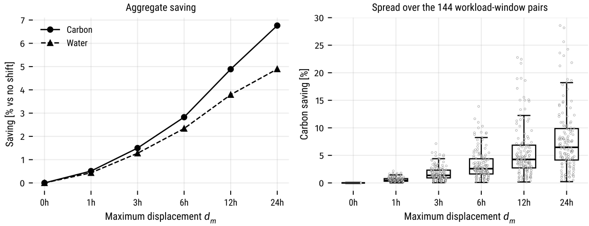
Figure 3.2: Ceiling of the static job-shifting analysis as a function of the maximum displacement d_m . The left panel shows the aggregate saving over all workloads and windows for each signal. The right panel shows the spread of the carbon saving across the 144 workload and window pairs.
