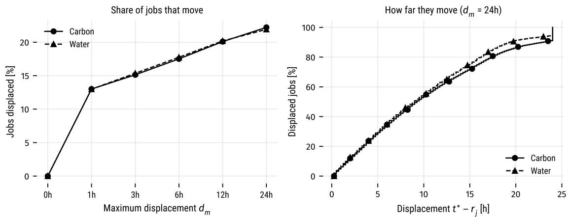
Figure 3.4: Share of jobs the static analysis displaces as a function of d_m (left) and the distribution of the displacement t^* - r_j among displaced jobs at a d_m of 24 hours (right).
