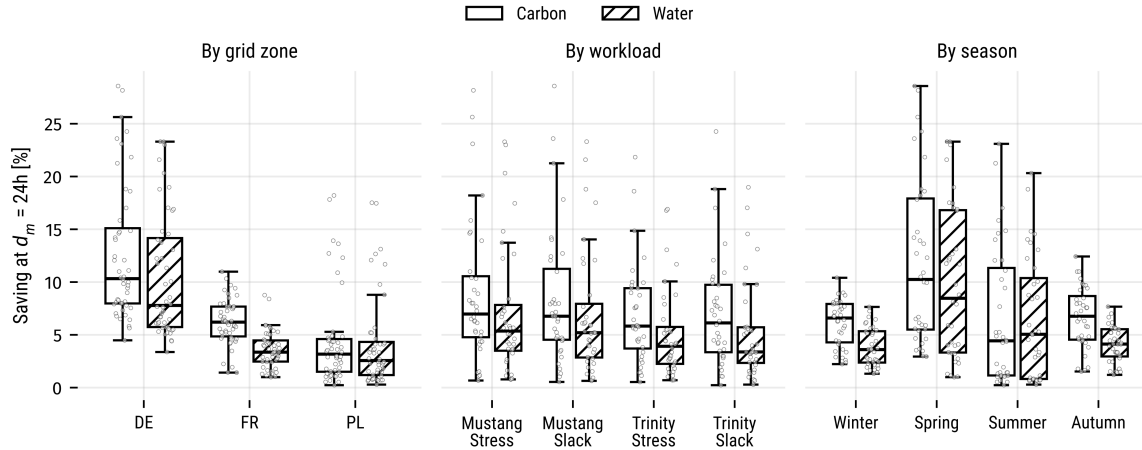
Figure 4.3: Ceiling at a d_m of 24 hours across the 144 workload and window pairs, split by grid zone, workload scenario, and season.
