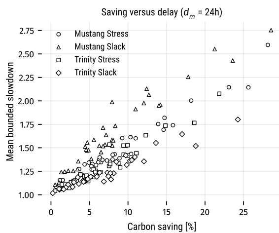
Figure 3.7: Carbon saving against mean bounded slowdown at a d_m of 24 hours, one point per workload and window pair.
