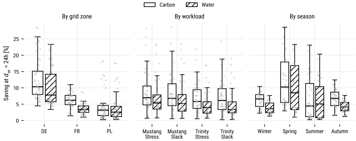
Figure 3.4: Ceiling at a d_m of 24 hours across the 144 workload and window pairs, split by grid zone, workload scenario, and season.
