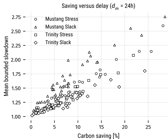
Figure 3.6: Carbon saving against mean bounded slowdown at a d_m of 24 hours, one point per workload and window pair.
