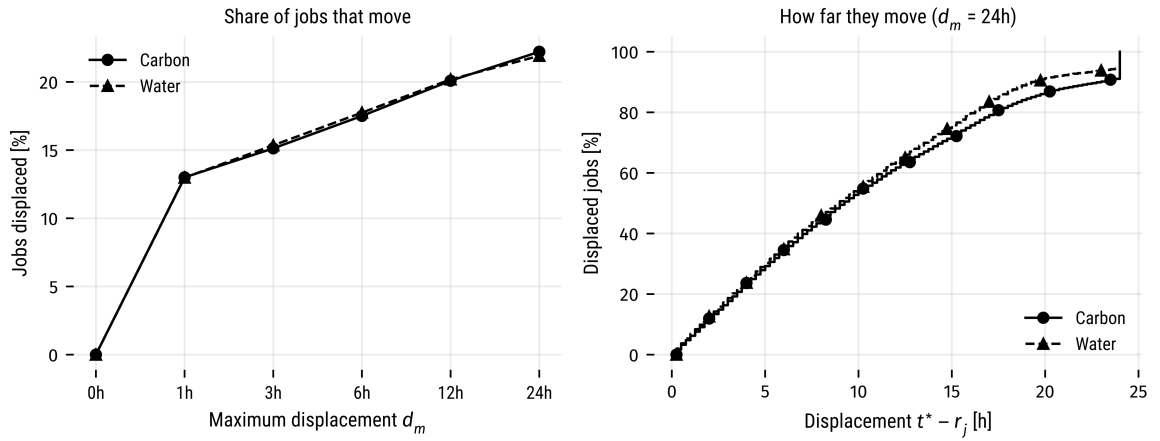
Figure 3.4: Share of jobs the offline analysis displaces as a function of d_m (left) and the distribution of the displacement t^* - r_j among displaced jobs at a d_m of 24 hours (right).
