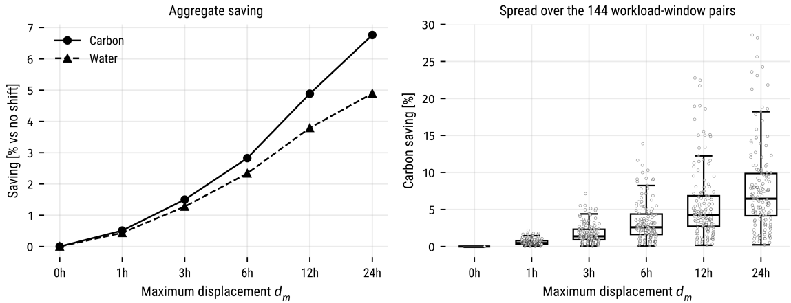
Figure 3.2: Ceiling of the offline job-shifting analysis as a function of the maximum displacement d_m . The left panel shows the aggregate saving over all workloads and windows for each signal. The right panel shows the spread of the carbon saving across the 144 workload and window pairs.
