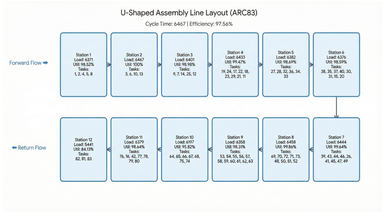
Figure 3: U-shaped assembly line layout for ARC83.IN2 obtained by the GA.
