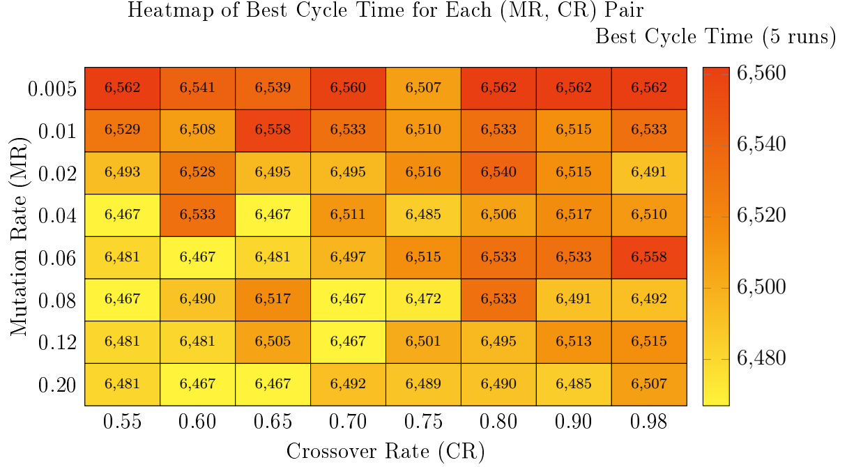
Figure 1: Heatmap of the best cycle time for each mutation crossover combination run for instance ARC83.
