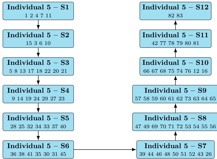
Figure 5: U-shaped 12-station assignment for ARC83 (Individual 5, Fitness = 0.000151).
