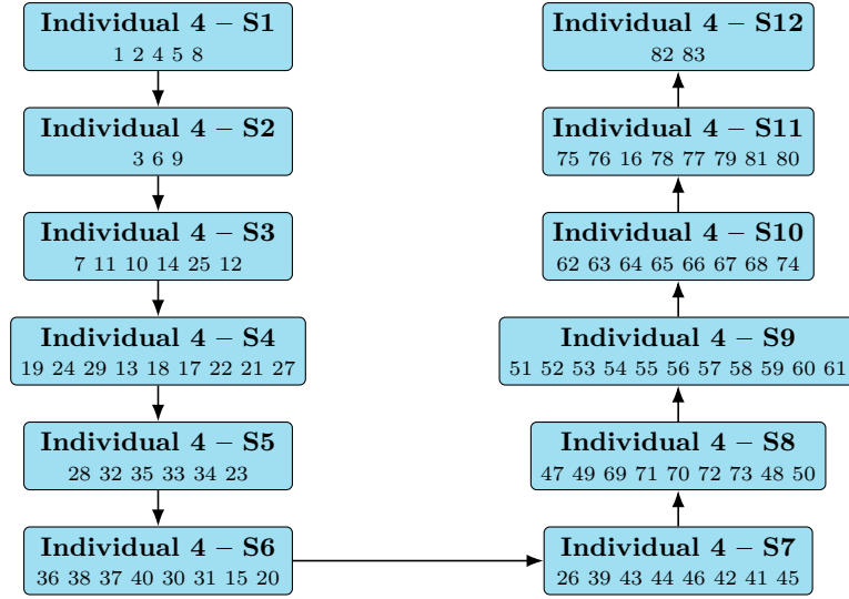
Figure 4: U-shaped 12-station assignment for ARC83 (Individual 4, Fitness = 0.000152).
