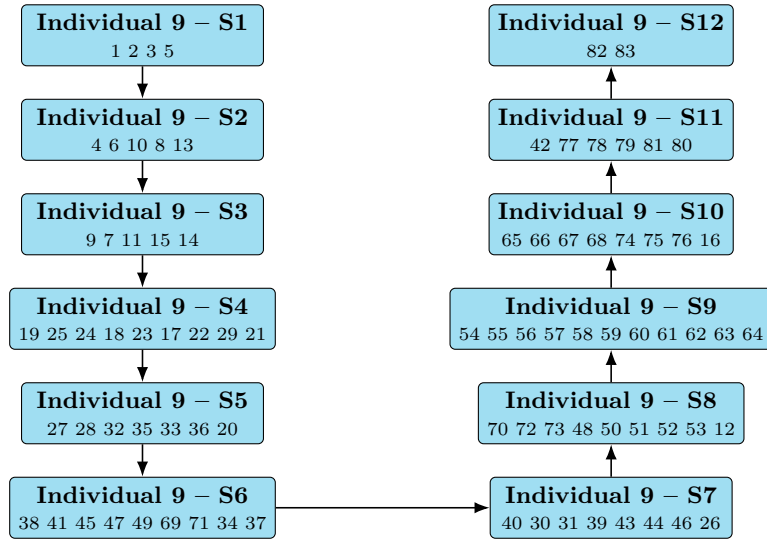
Figure 9: U-shaped 12-station assignment for ARC83 (Individual 9, Fitness = 0.000151).
