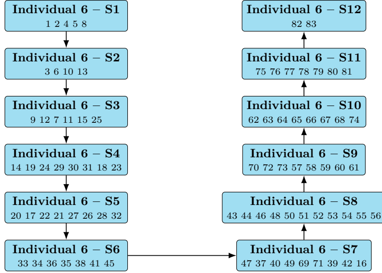
Figure 6: U-shaped 12-station assignment for ARC83 (Individual 6, Fitness = 0.000151).
