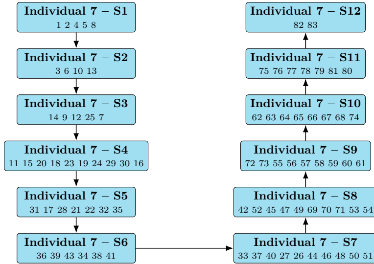
Figure 7: U-shaped 12-station assignment for ARC83 (Individual 7, Fitness = 0.000151).
