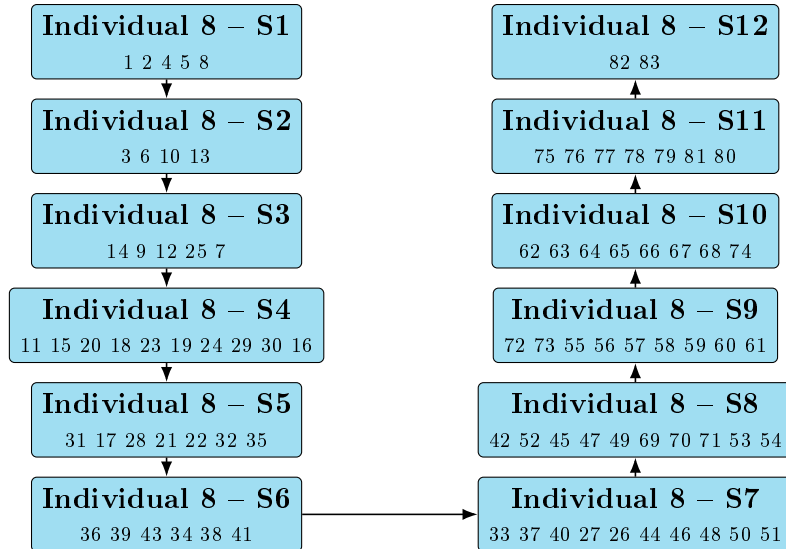
Figure 17: U-shaped 12-station assignment for ARC83 (Individual 8, Fitness = 0.000151).
