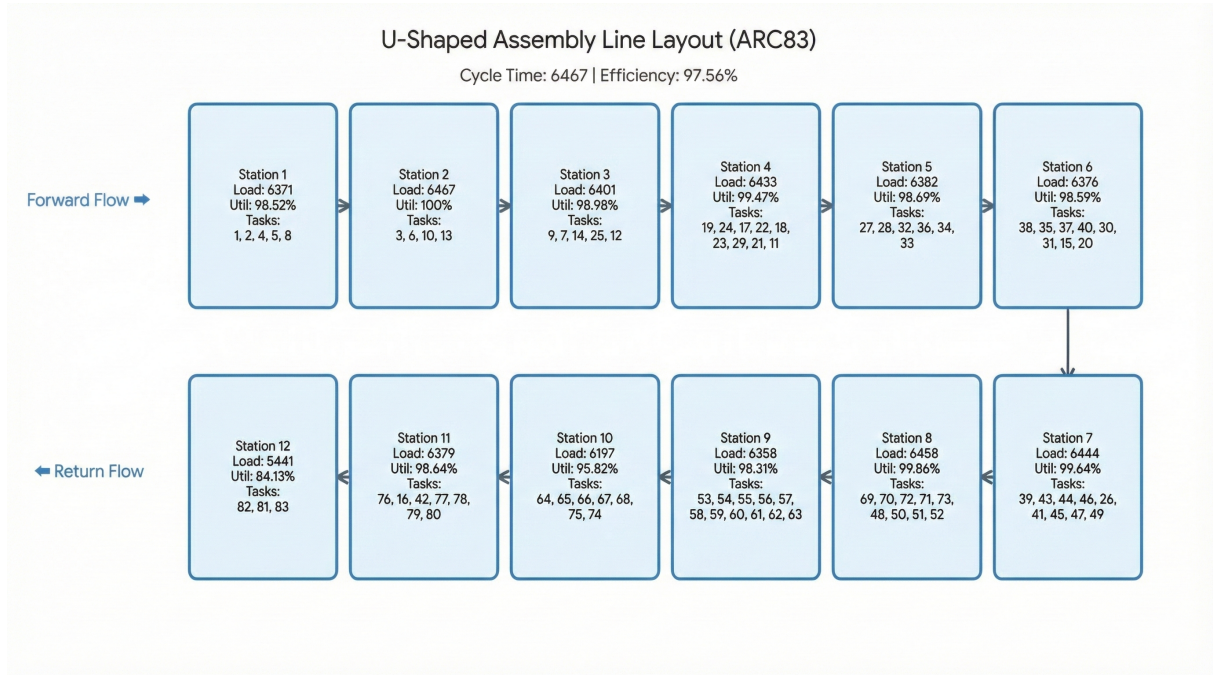
Figure 9: U-shaped assembly line layout for ARC83.IN2 obtained by the GA.
