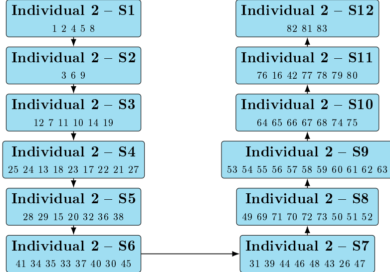
Figure 8: U-shaped 12-station assignment for ARC83 (Individual 2, Fitness = 0.000153).
