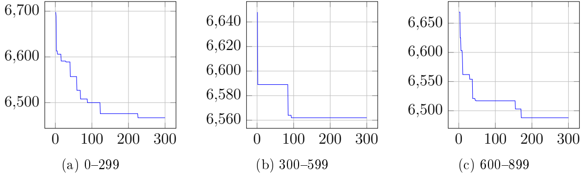
Figure 3: Convergence graphs for ARC83 (Best cycle time so far) - Part 1
