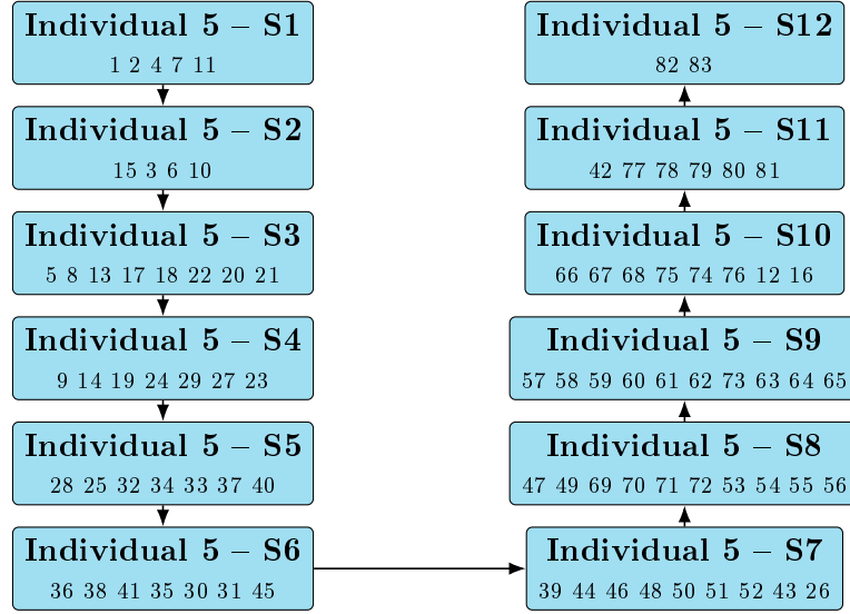
Figure 14: U-shaped 12-station assignment for ARC83 (Individual 5, Fitness = 0.000151).
