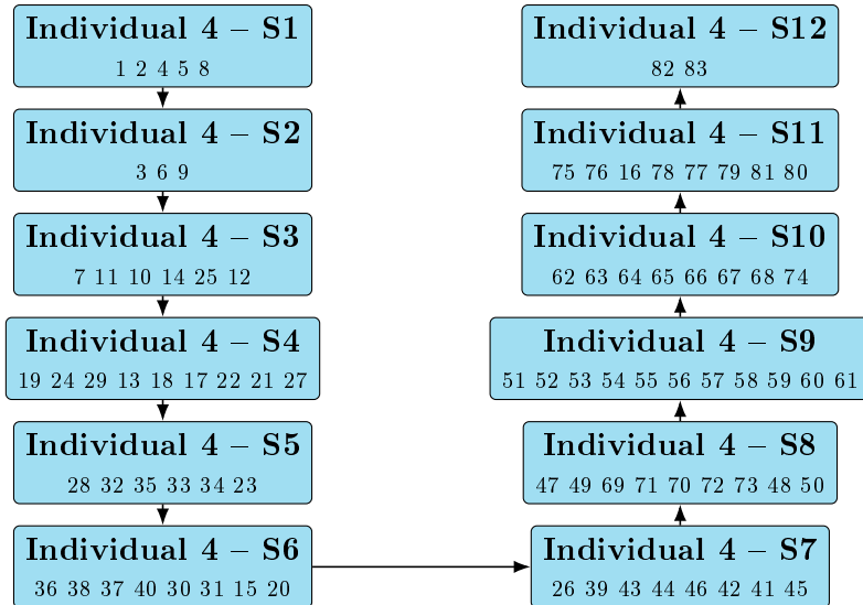
Figure 13: U-shaped 12-station assignment for ARC83 (Individual 4, Fitness = 0.000152).
