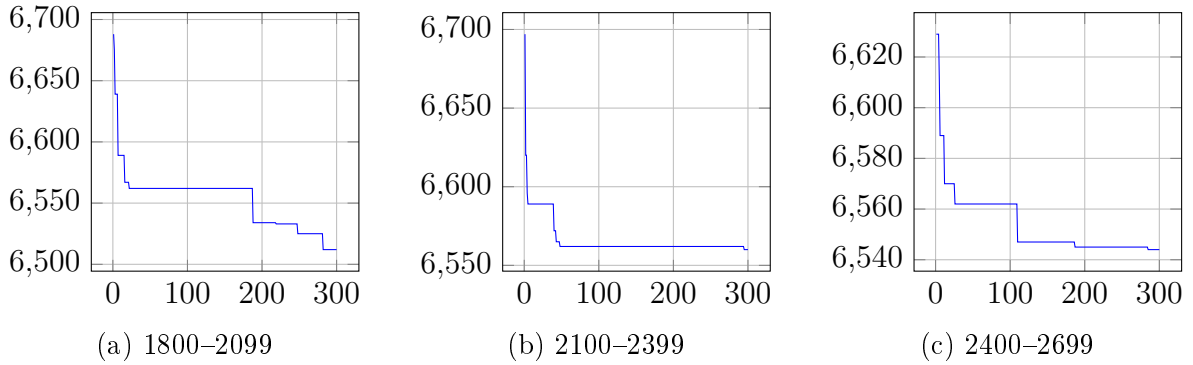
Figure 5: Convergence graphs for ARC83 (Best cycle time so far) - Part 3
