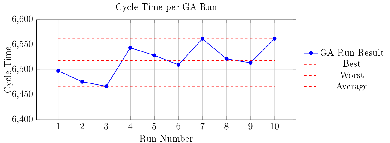
Figure 4: Instance ARC83 cycle time obtained in each of the 10 independent GA runs, including best, worst, and average values.
