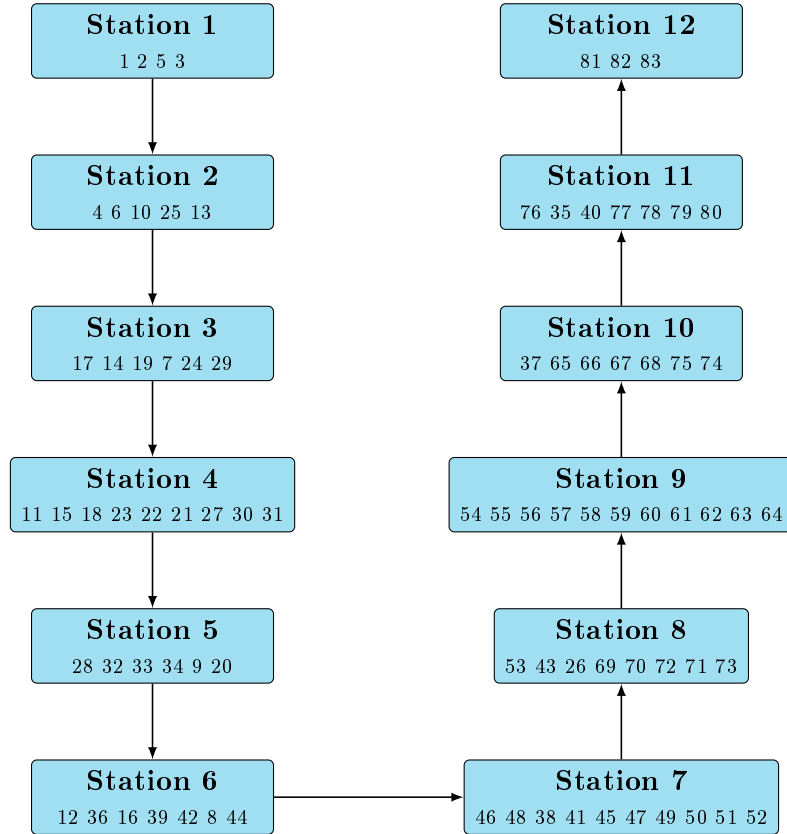
Figure 13: U-shaped 12-station assignment for ARC83 (Individual 6, Fitness = 0.000155).
