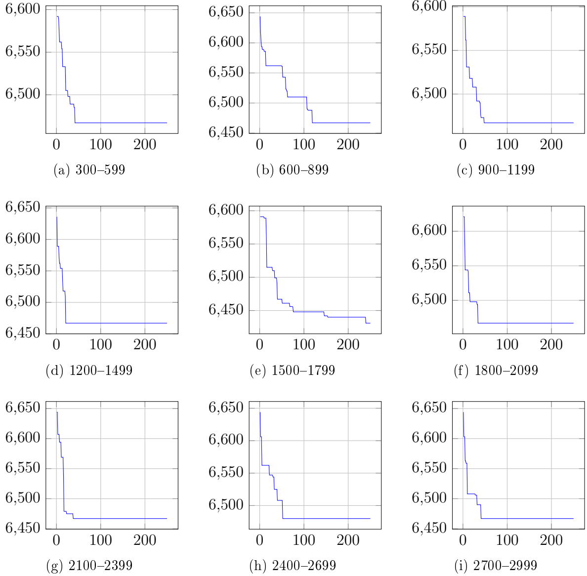
Figure 3: Convergence graphs for ARC83 (Best cycle time so far)
