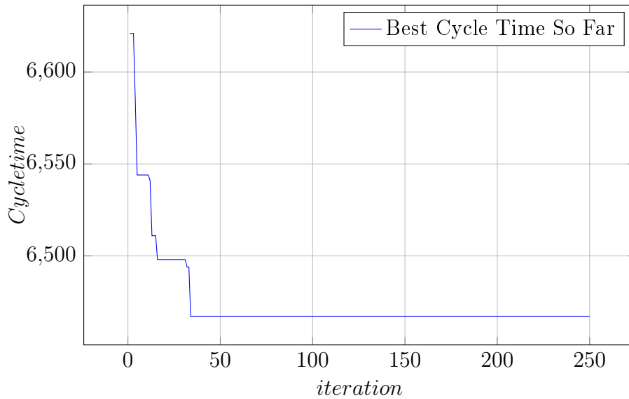
Figure 2: Convergence graph for ARC83
