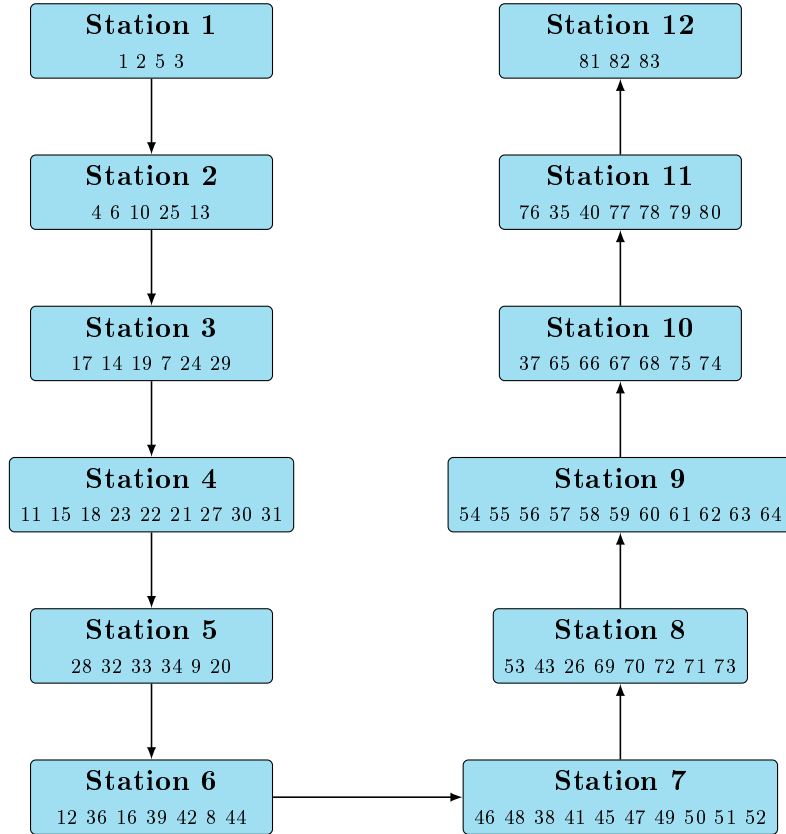
Figure 12: U-shaped 12-station assignment for ARC83 (Individual 5, Fitness = 0.000155).
