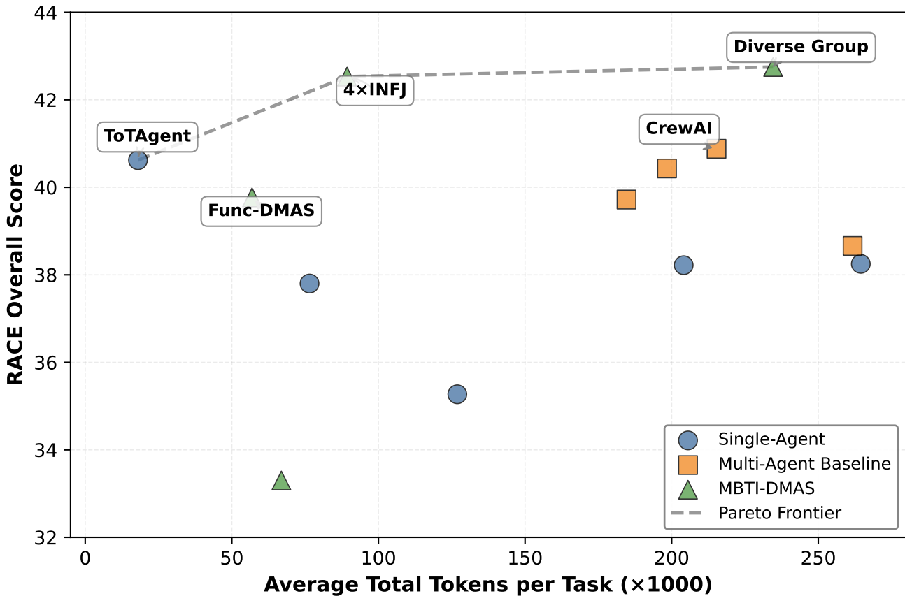
Efficiency-Quality Pareto Frontier
