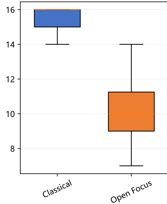
Observed states
