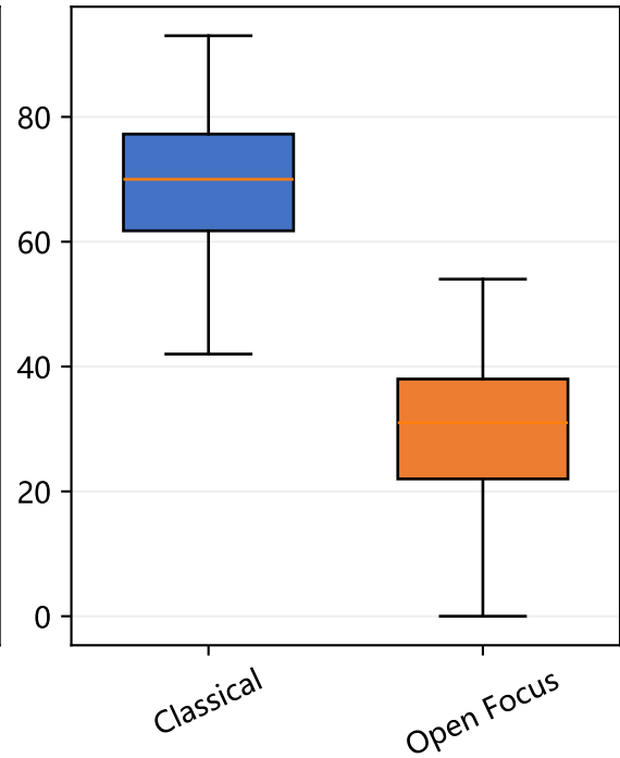
Directed edges
