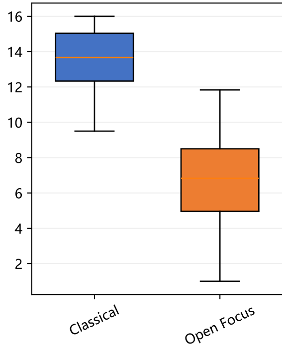
Mean beta0
