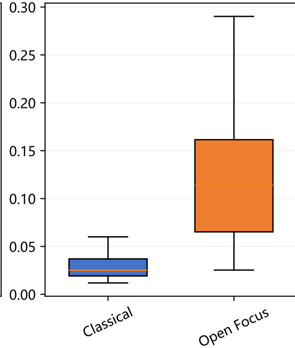
Directed recurrence
