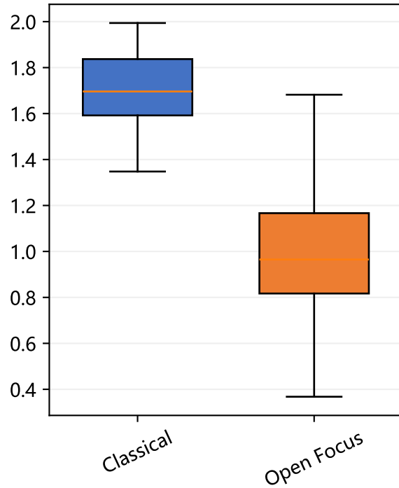
Path entropy
