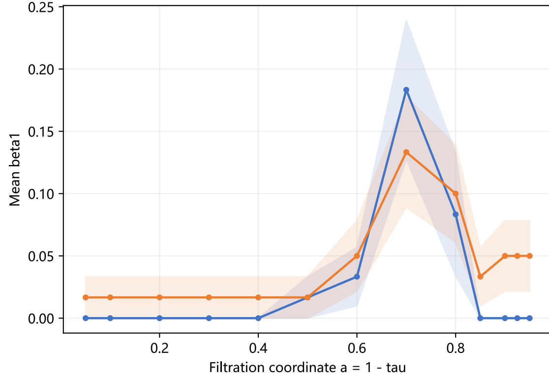
Mean beta1
