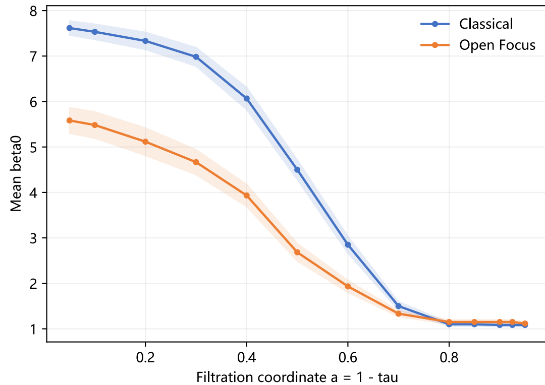
Mean beta0
