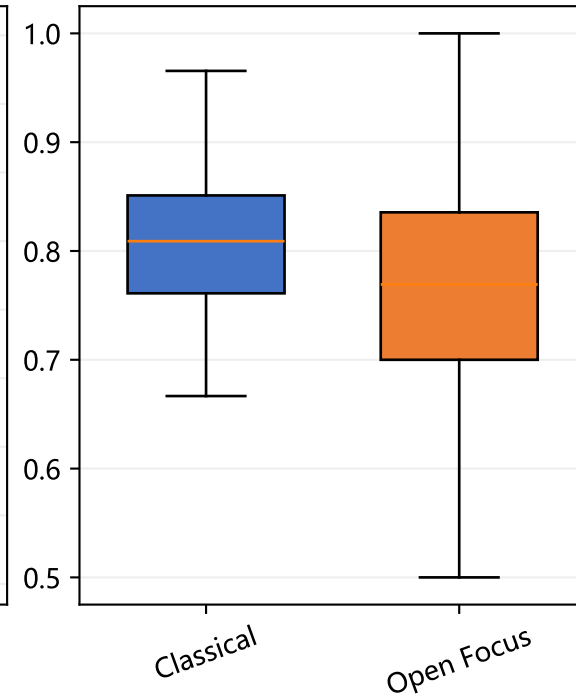
Reciprocity
