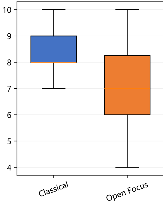
Observed states
