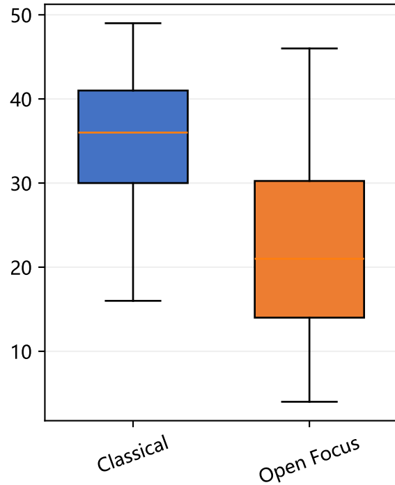
Directed edges
