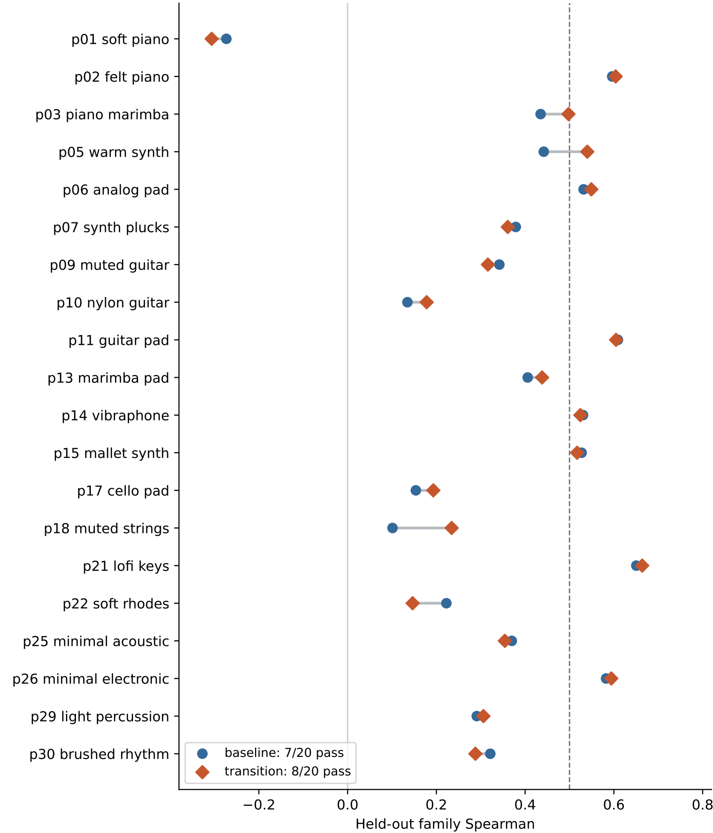
Three-seed energy ensemble: 20 train families
