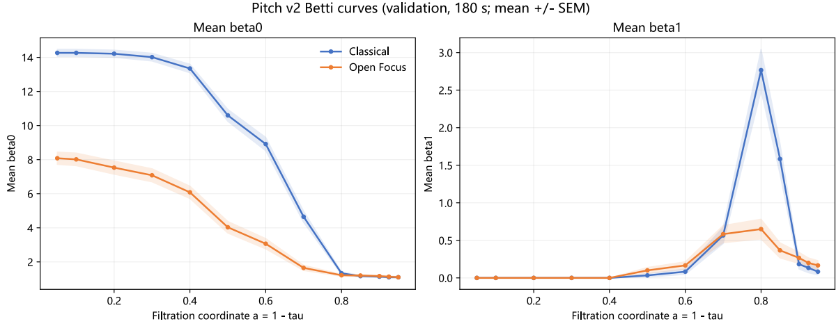
Figure 11: Betti curves of the pitch view.
