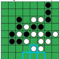
Adjacent NoFlip
