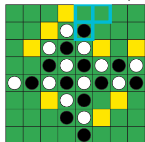
Standard NoFlip
