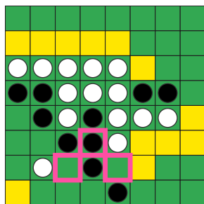
Edited GT
