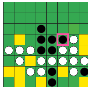
GS
