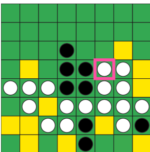
Unedited Pred
