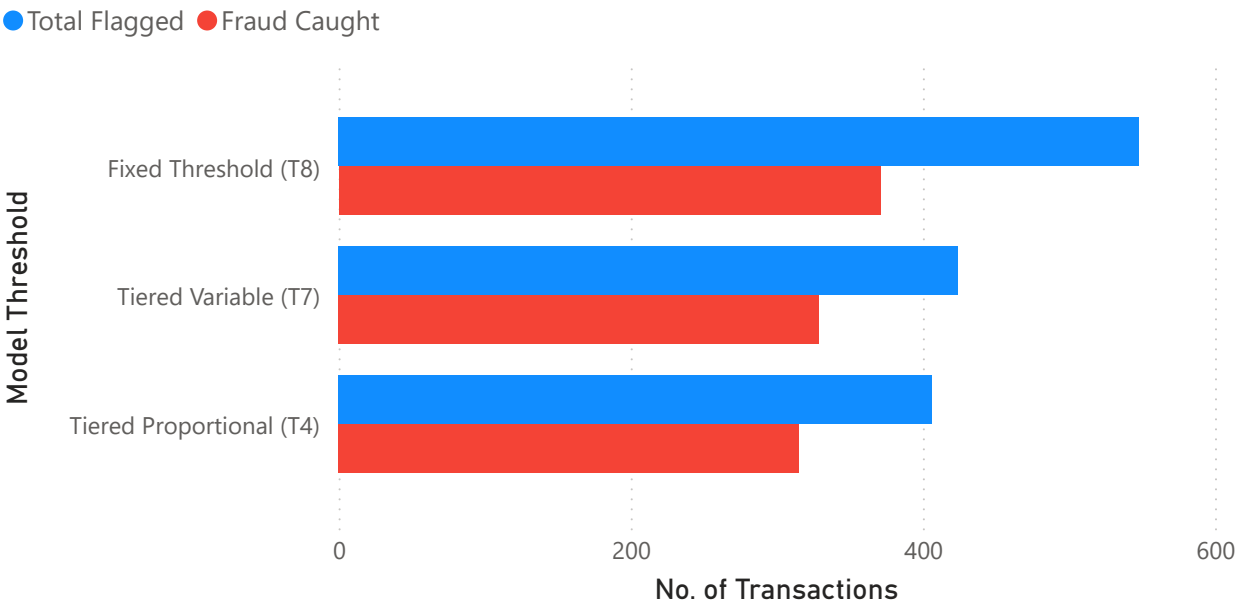
Flagged vs Fraud Caught
