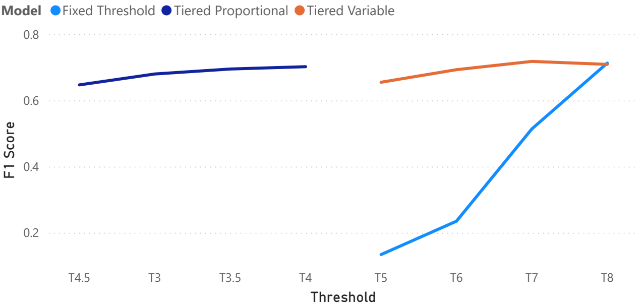
F1 Score Across Thresholds
